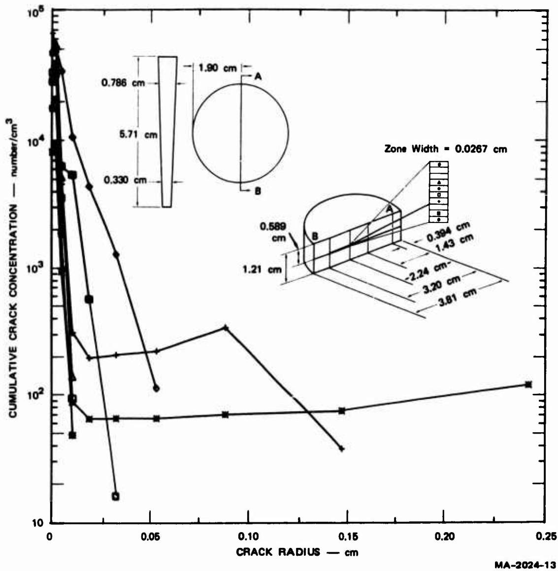
FIGURE 11 CRACK SIZE DISTRIBUTIONS ON SECTION A-B, FILE 3 OF SPECIMEN 2024-4
