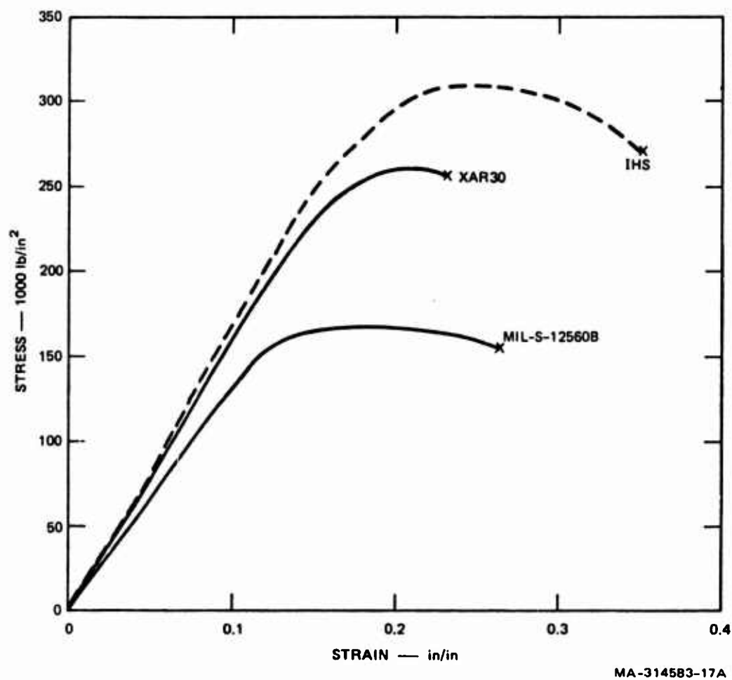
FIGURE E-2 STRESS-STRAIN CURVES FROM SHORT TRANSVERSE TENSILE TESTS OF THREE ARMOR STEELS
