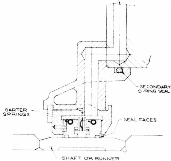
Fig. 6.1 -- Schematic of typical tandem circumferential seal
