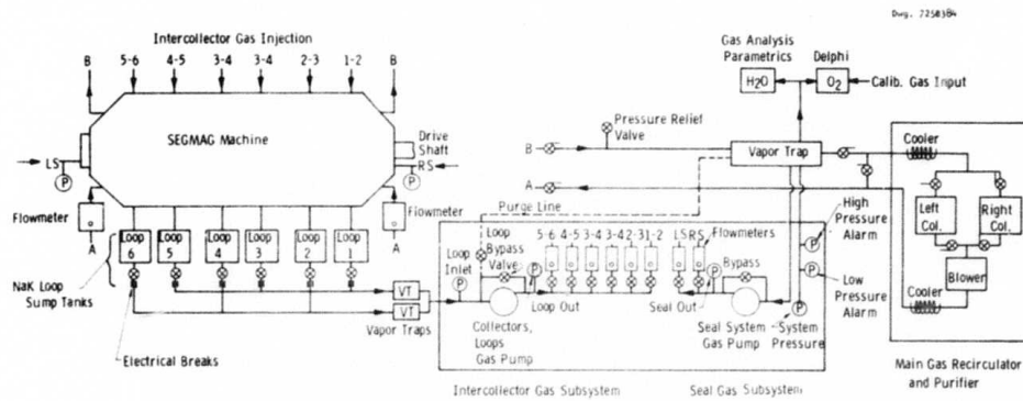
Fig. 5.3: SEGMAG cover gas systems
