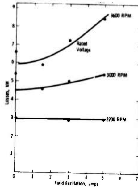
Fig. 2.2.9: GEC calculated MHD losses.
