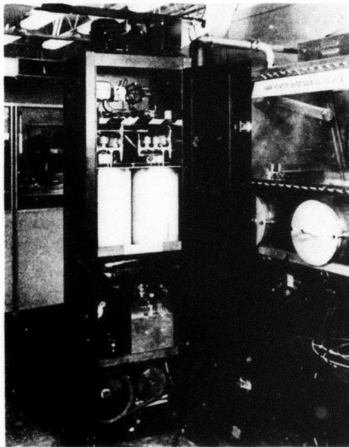
Fig. 5.4: Internal components of central gas purifier station for the SEGMAG homopolar machine
