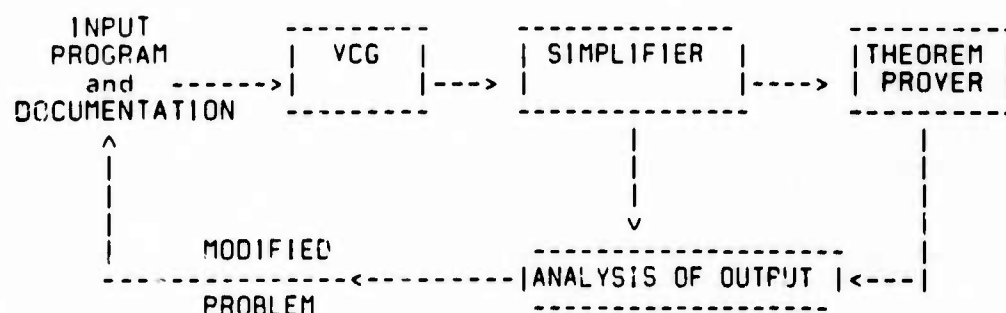
Figure 1: Main Components of the Verifier
