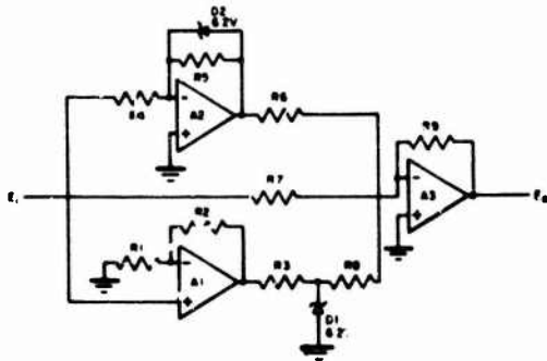
Figure 2. Shaping Circuit.
