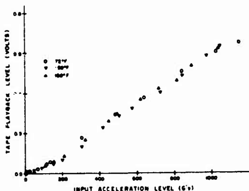
Figure 5. System Performance.
