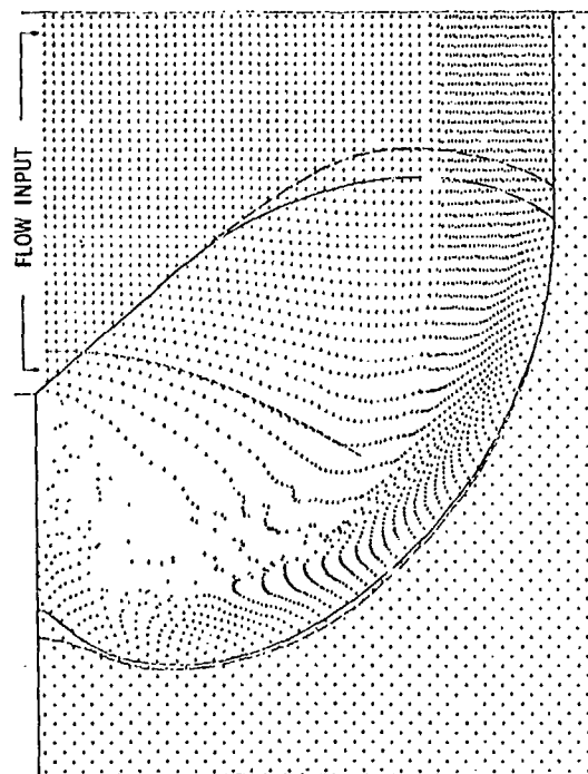
Figure 4-12. Configuration of Mass Points at Time t = 6.329 for the Calculation for Nitrogen With M_s = 1.588
