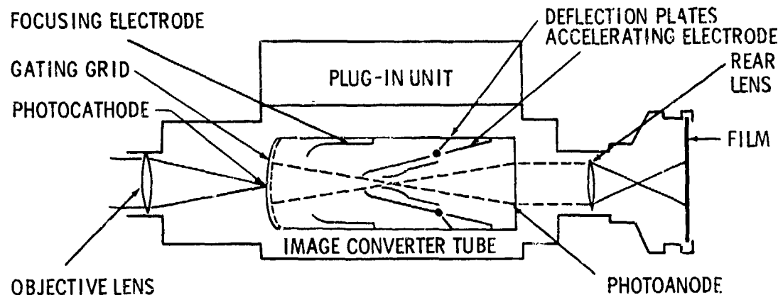
Figure 9-16. Schematic of Image-converter Camera (Courtesy of STL)
