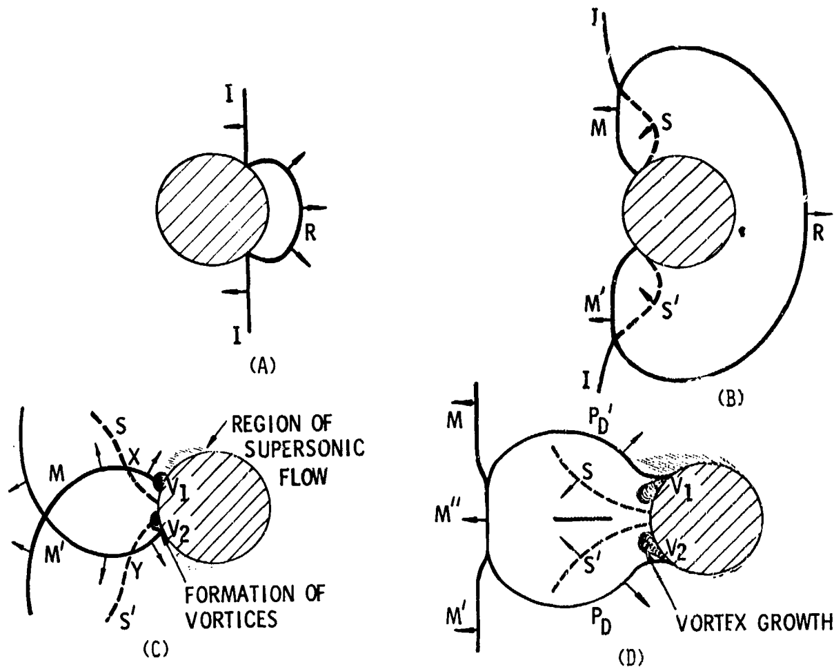
Figure 1-14. Tracings of Shadowgraphs Showing the Interaction of a Shock Front With a Cylinder
