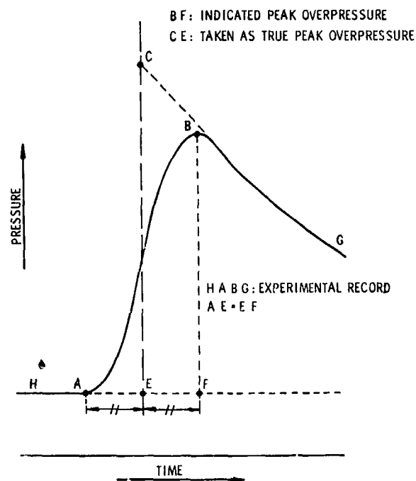
Figure 10-5. Method of Extrapolation of Experimental Records
