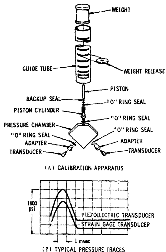
Figure 8-15. Dynamic Pressure Calibrator of Rathke 16
