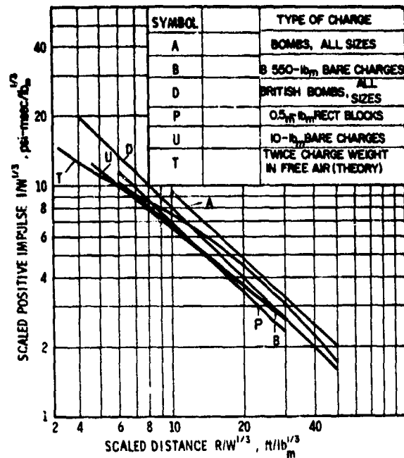
Figure 3-3. Experimental Positive Impulses vs Distance Curves (on ground) from Various Sources 4
