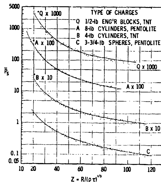
Figure 5-3. Experimental Pressure vs Scaled Distance for Four Types of Charges 2
