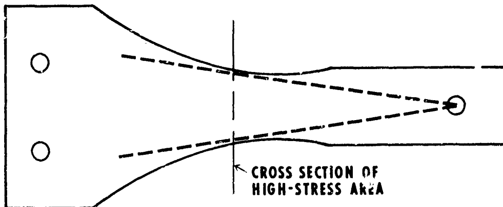
Figure 1. Specimen configuration.
