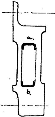
SECTION-SPROCKET BEARING SURFACE NOS. 2 & 3 (a. .008"/.018" b. .006"/.016")
