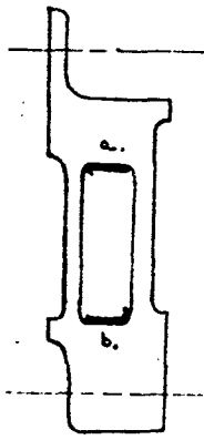
SECTION-SPROCKET BEARING SURFACE Nos. 2 & 3 (a. .010"-.020") (b. .014"-.020")
