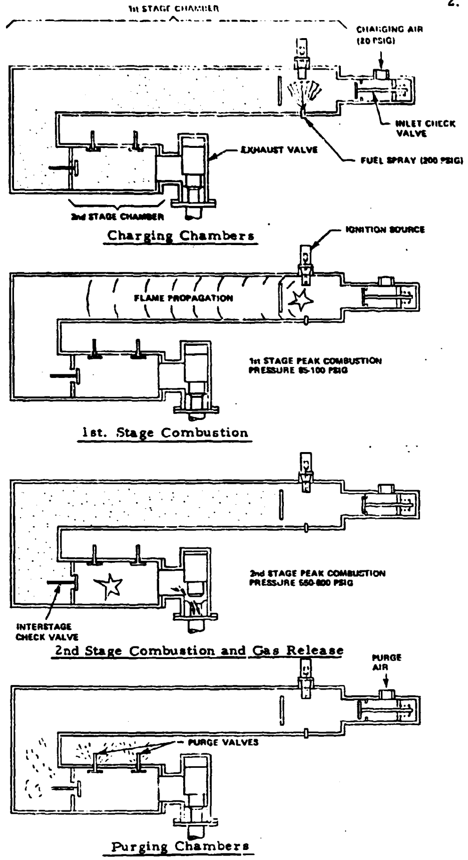
FIGURE 1. TWO-STAGE COMBUSTION OPERATING SEQUENCE
