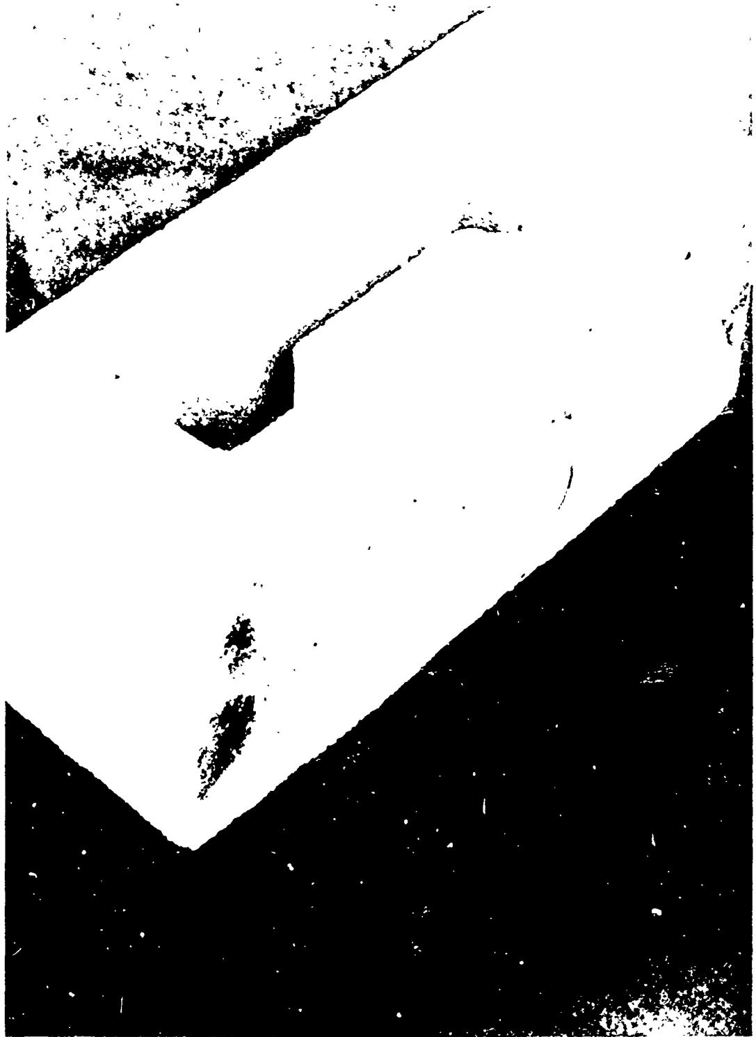
Figure 12. Ceramic Riser configuration on top of permanent mold.
