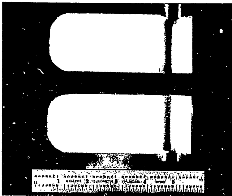
Figure 30. Austenitic grey iron mold. Mold is identical in shape to that in Fig. 22. Interior of mold plasma-sprayed with ZrO_2 .
