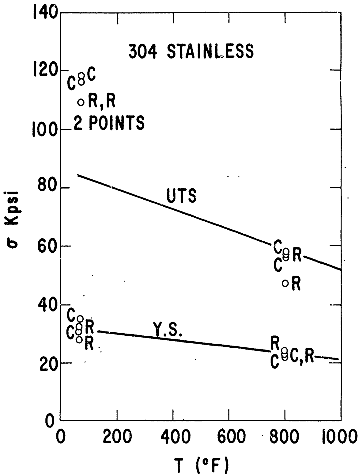
Figure 49. Tensile properties of conventional and rheocast 304 stainless steel.
