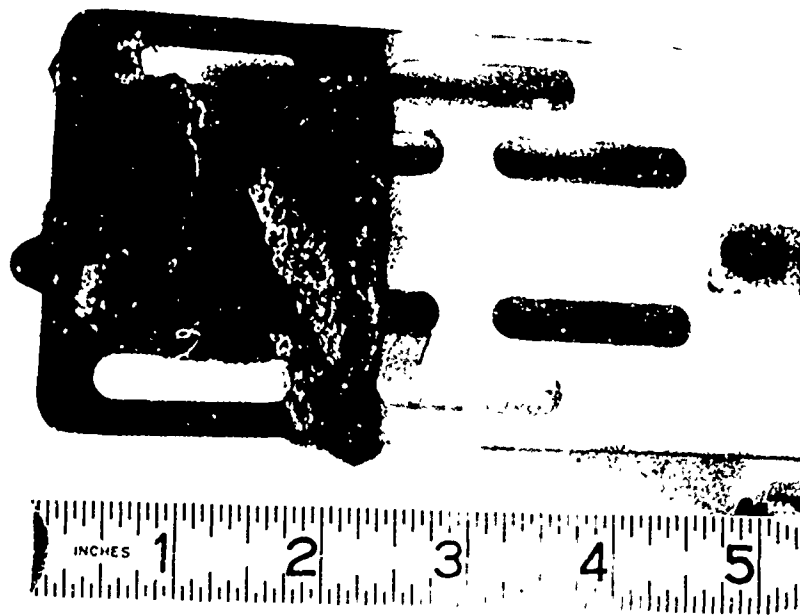
Figure 34. ZrO_2 sprayed molybdenum paddle. Metal mechanically adhering, but no penetration of coating.
