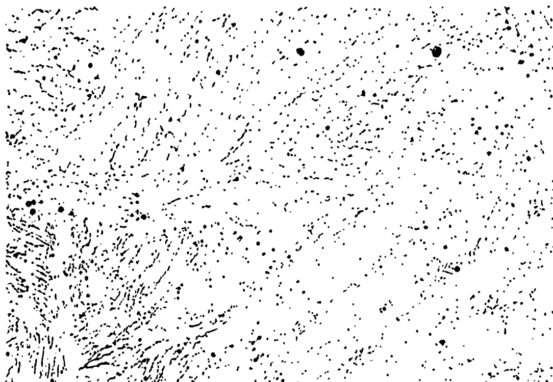
(b) conventional permanent mold cast 150X
