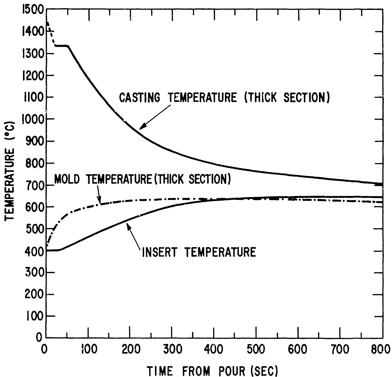
Figure 16. Thermocouple data showing casting temperature, mold temperature, and temperature of insert. Alloy cast was Mar M-502, mold temperature 400°C, pouring temperature 1435°C.
