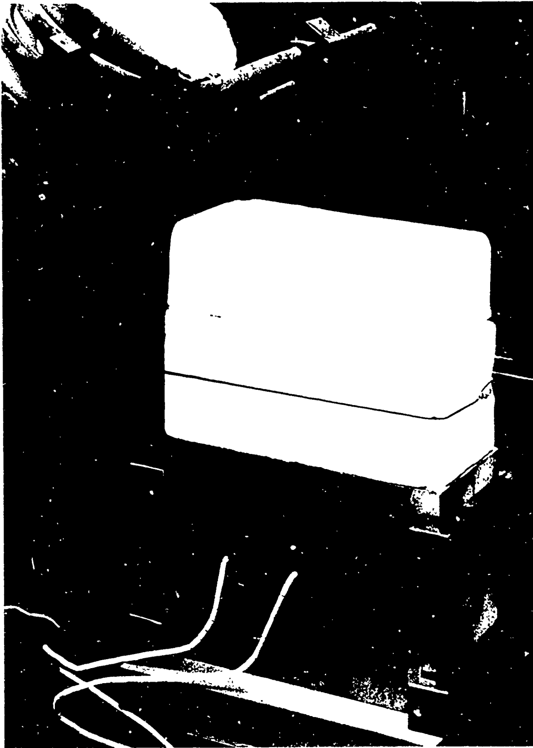
Figure 13. Furnace arrangement: mold, pouring basin, and riser. Thermocouples extending out of mold monitor melt temperature, mold temperature, and insert temperature. Mold arrangement is surrounded by heater in actual use.
