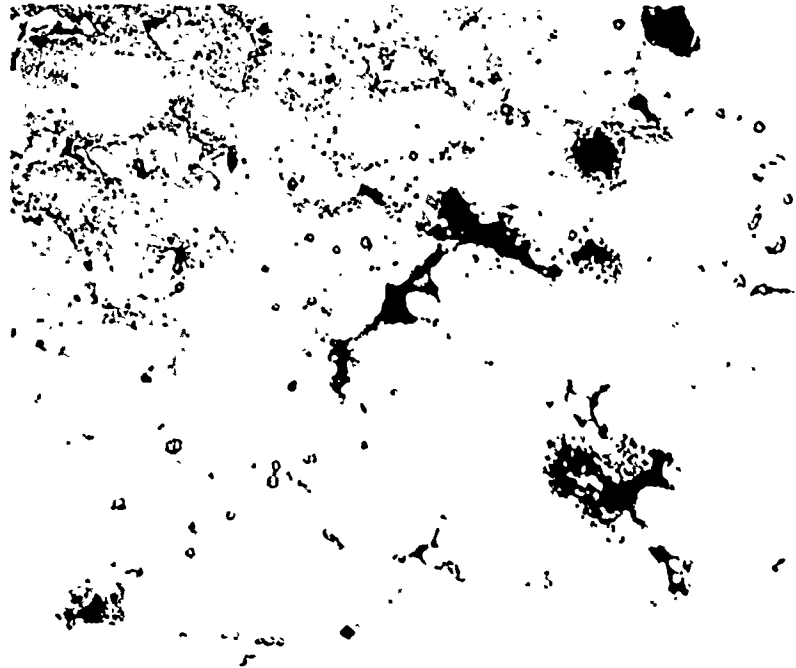
Figure 21. TRW VI A casting same as Figs. 19 and 20. Microporosity associated with \gamma - \gamma' eutectic. Marble's reagent. 250X
