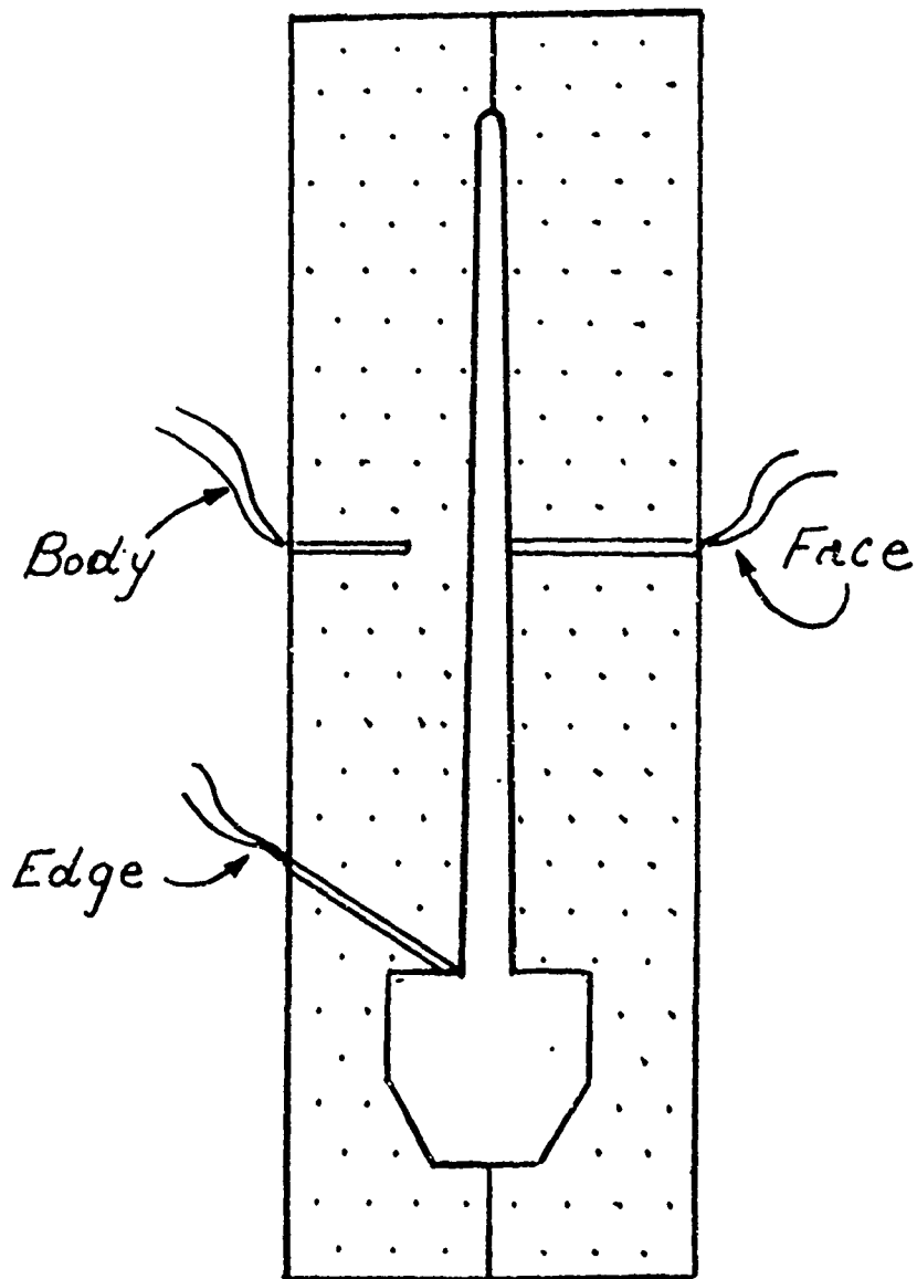
Figure 31. Schematic of grey iron blade mold showing position of thermocouples. Thermocouples on face and edge positions welded to inside mold face.
