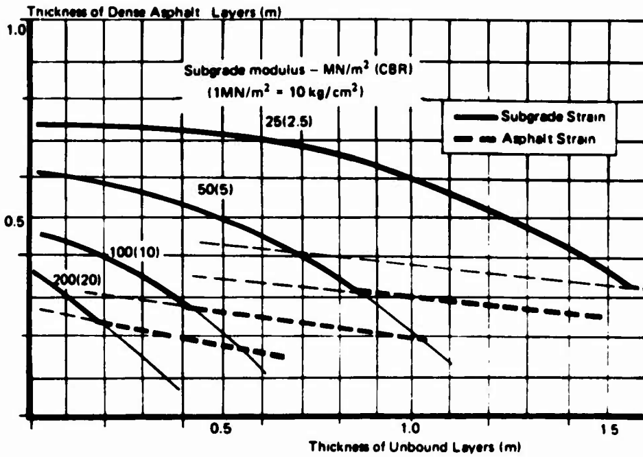
Fig. G9a Design curves for B707-3208 (Edwards and Valkering, 1970)
