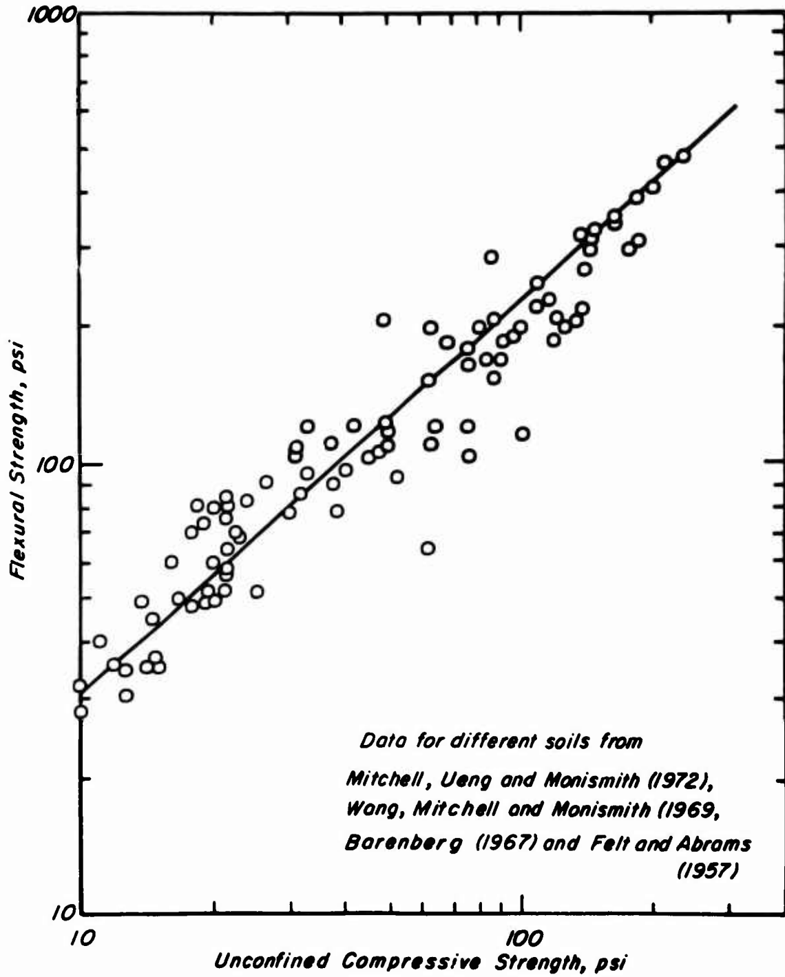
Fig. 8 The relation between the unconfined compressive strength and the flexural strength of soil and cement mixtures
