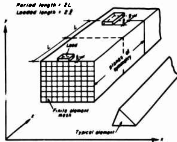
Fig. B4 Prismatic space finite element representation
