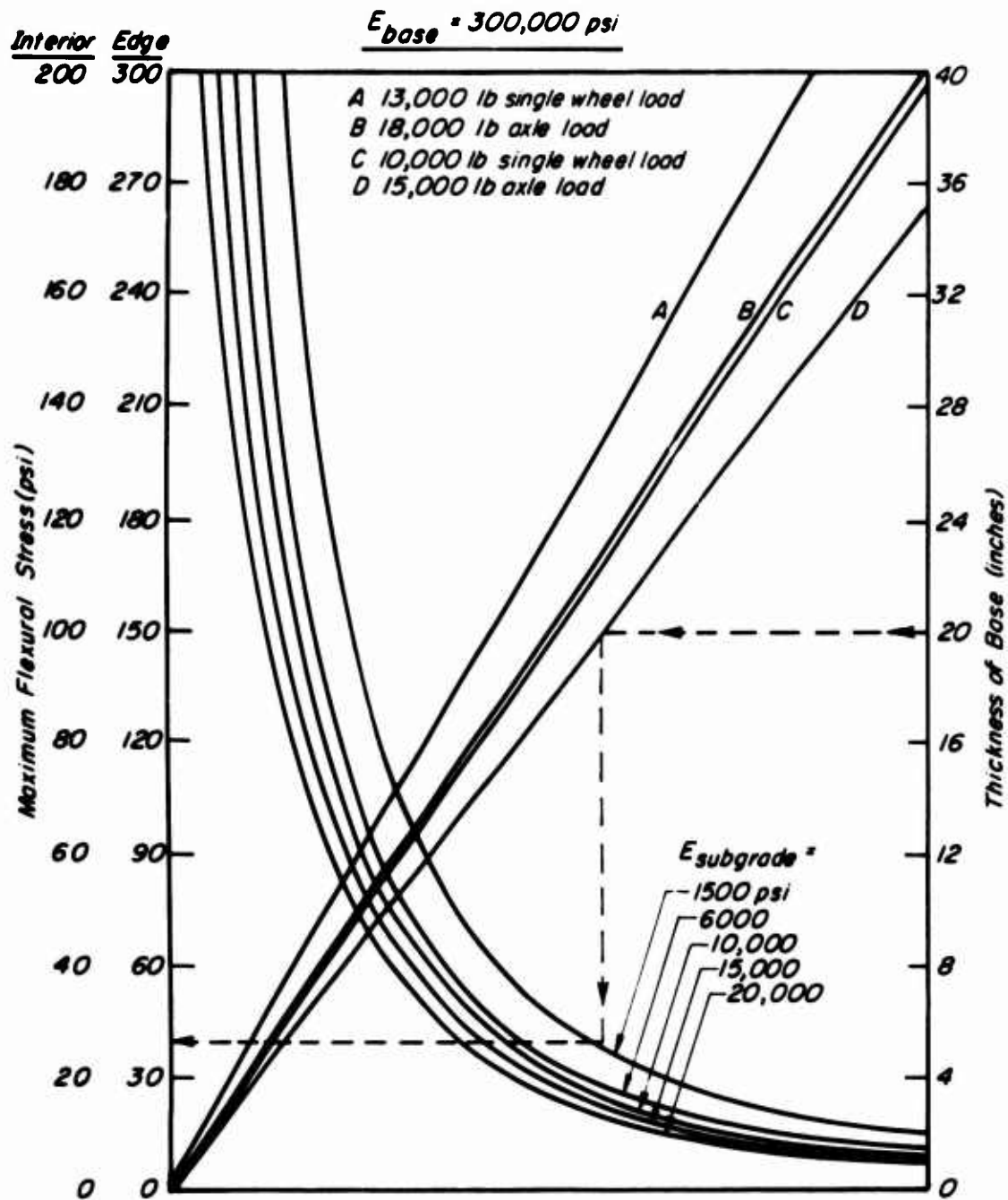
Fig. 18 Relationship between tensile stress and base thickness for various single and dual-wheel loads, E_{base} = 300,000 \text{ psi}
