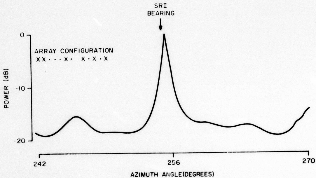
Figure 15. Comparison of Azimuth Maps of SRI Signal (15.729 MHz) with Filled Array (top) and Sparse Array (bottom). The Sparse Array has fewer elements but Comparable Aperture.
