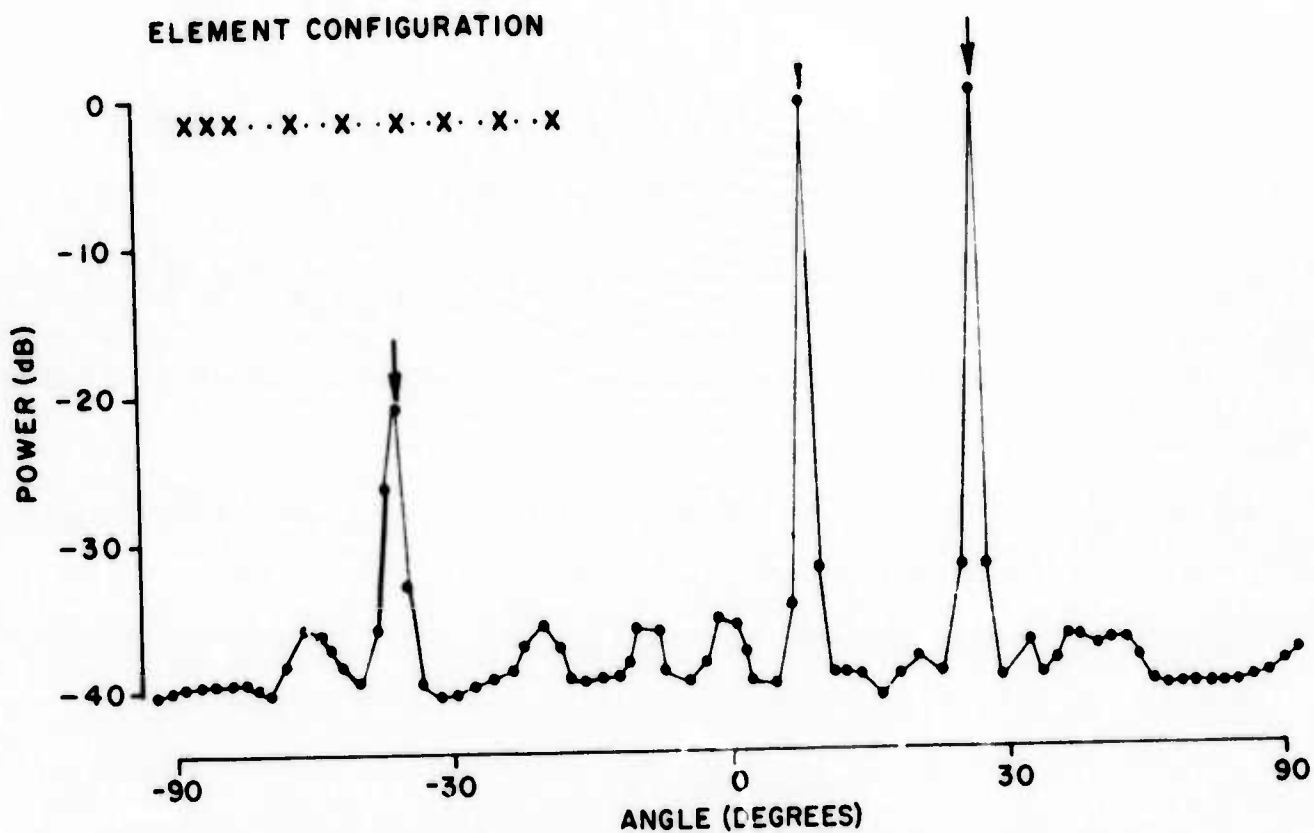
Figure 9. Comparison between the Adaptive Performance of a Sparse Array (bottom) and a Filled Array of the Same Number of Elements (top).
