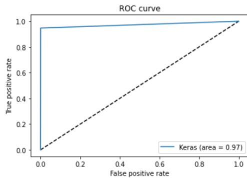
Figure 23 The GAN ROC and AUC
