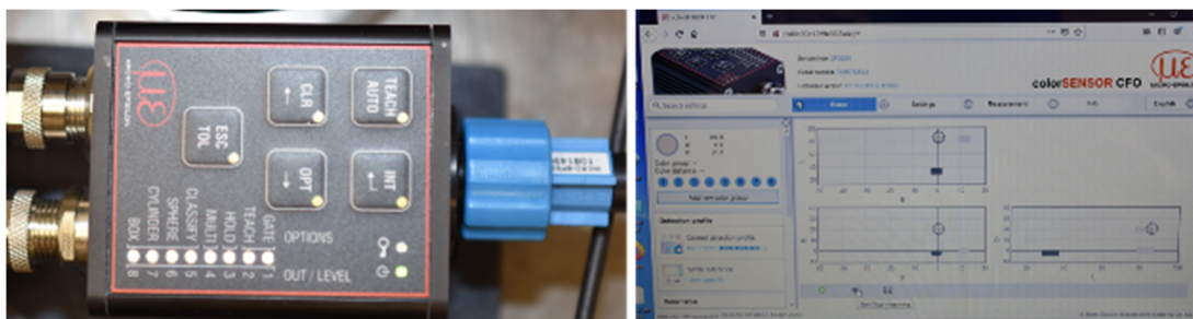
Figure 1. (Left) CFO200 sensor with fiber-optic and blue connector and (right) the graphical user interface, which operates within any browser through a direct Ethernet connection.
