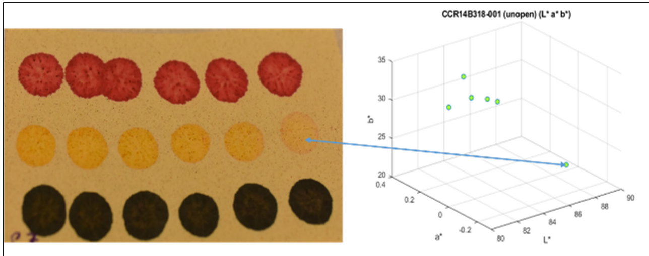
Figure 11. (Left) CCR14B318-001 (unopened) shows the sixth droplet of G being (right, center row) visibly lighter and (right) close-up of only the CCR14B318-001 (unopened) CIELAB values shows that the sixth point shifted in the a^* and b^* spaces.
