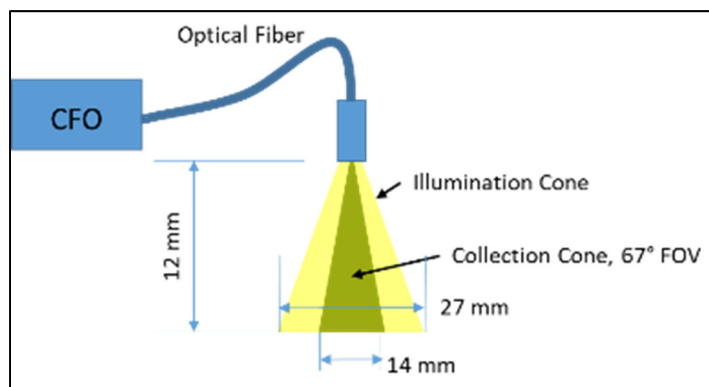
Figure 2. Schematic of data collection with the CFO200 sensor. All dimensions are approximate due to variation in paper flatness and, in the case of the illumination cone, qualitative perception of the lighted region.
