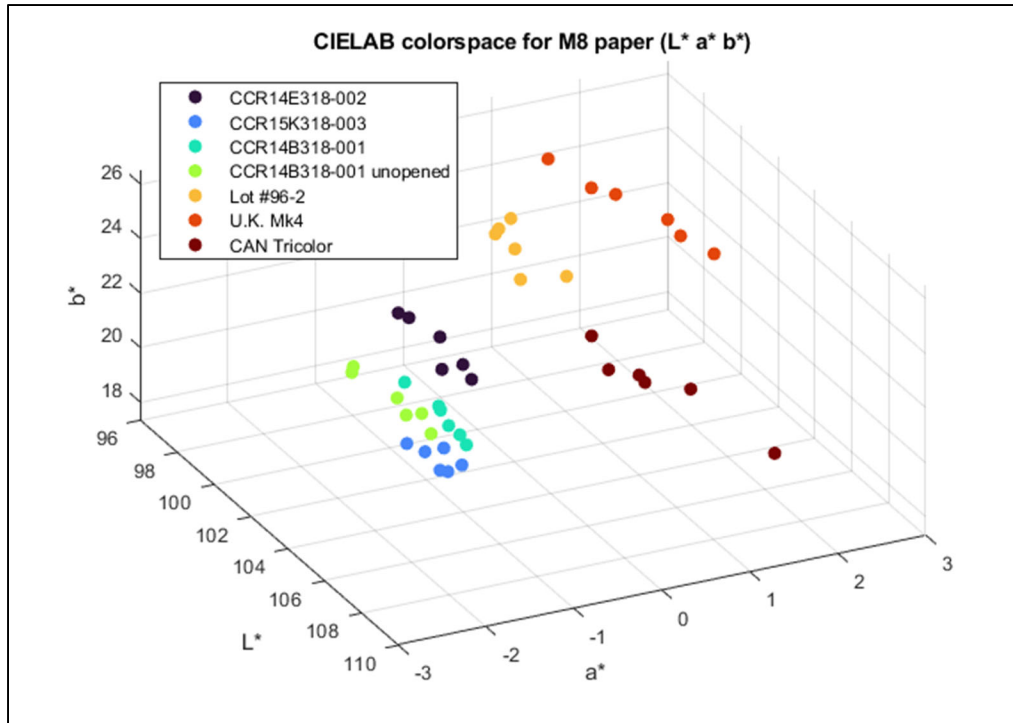
Figure 6. Measured baseline values for each paper sample in L*a*b* space.
