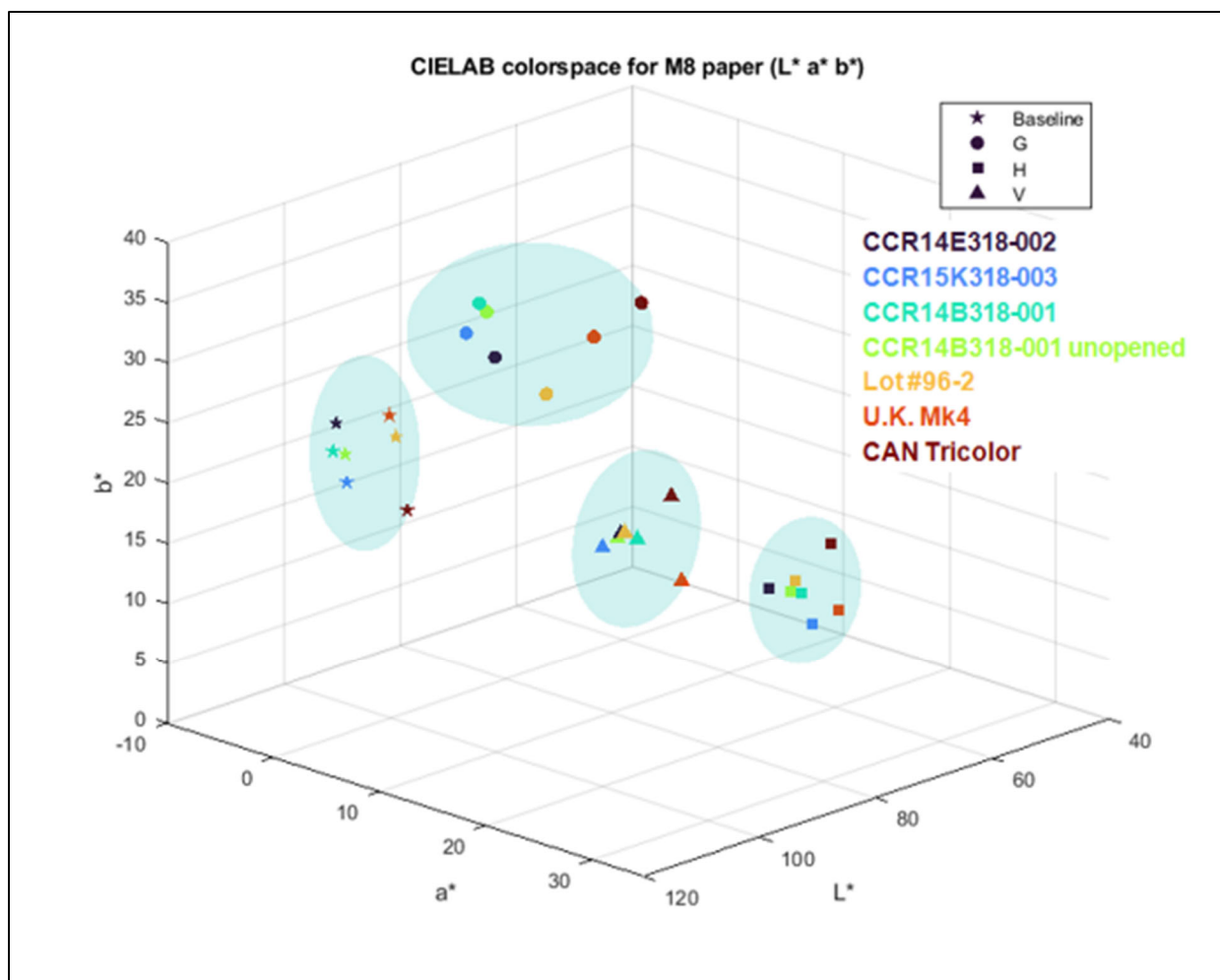
Figure 8. Average 3D space ( L^*a^*b^* ) locations for all seven paper types: unexposed (star) and exposed to agent classes G (circle), H (square), and V (triangle). Each is clearly clustered in a unique region of this 3D space.
