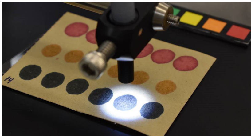
Figure 3. Collection of CIELAB data with CFO200 sensor.
