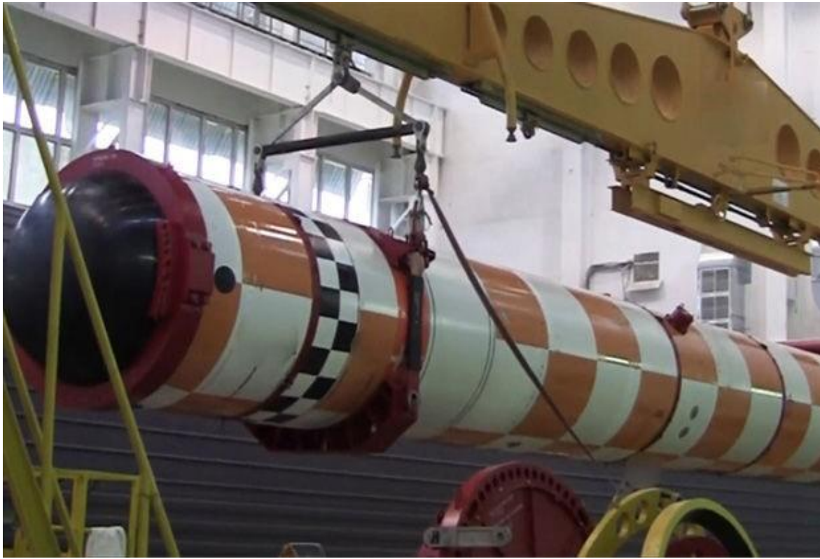
Figure 21. Poseidon UUV
