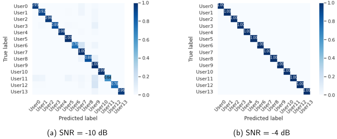
Figure 5.4. SGAN dense classifier performance with SNR at (a) -10 dB, (b) -4 dB. Source: [38].
