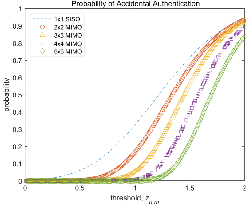
Figure 3.3. Probability of authentication for various MIMO configurations and thresholds. Source: [87].
