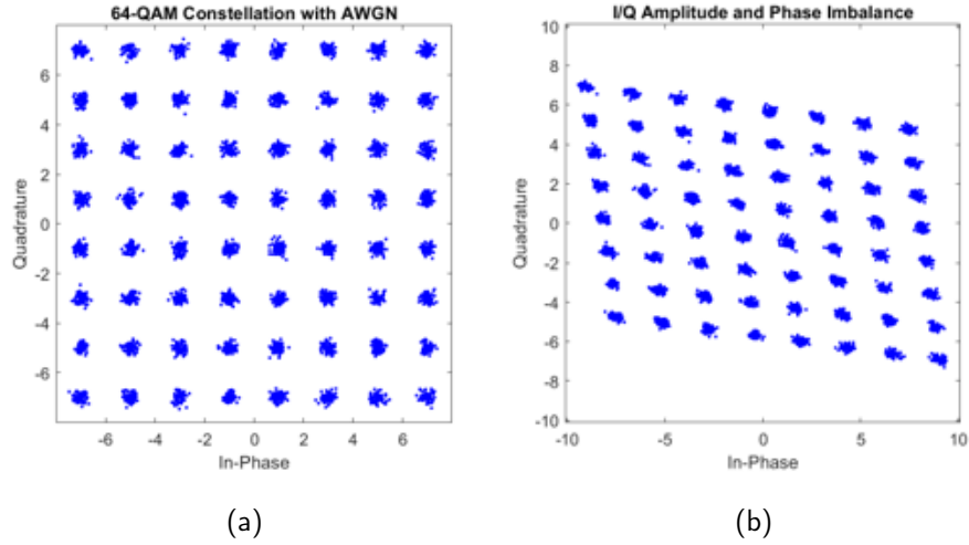
Figure 1.2. Amplitude and IQ imbalance for 64-QAM (a) before and (b) after 3 dB amplitude and 15 degree phase imbalance.
