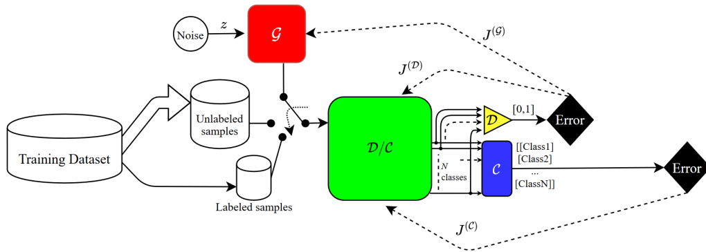
Figure 1.8. Training a semi-supervised generative adversarial network with N classes. Adapted from [38].
