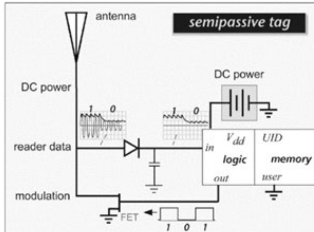
Figure 3. Semi-Passive RFID Tag. Source: Dobkin (2007).
