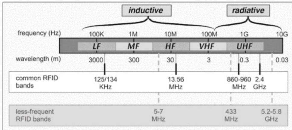
Figure 1. RFID Electromagnetic Spectrum use. Source: Dobkin (2007).
