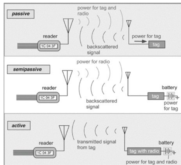
Figure 2. RFID Tag Configuration. Source: Dobkin (2007).
