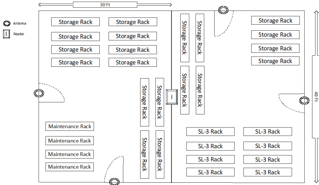
Figure 12. Sample Company RFID Implementation
