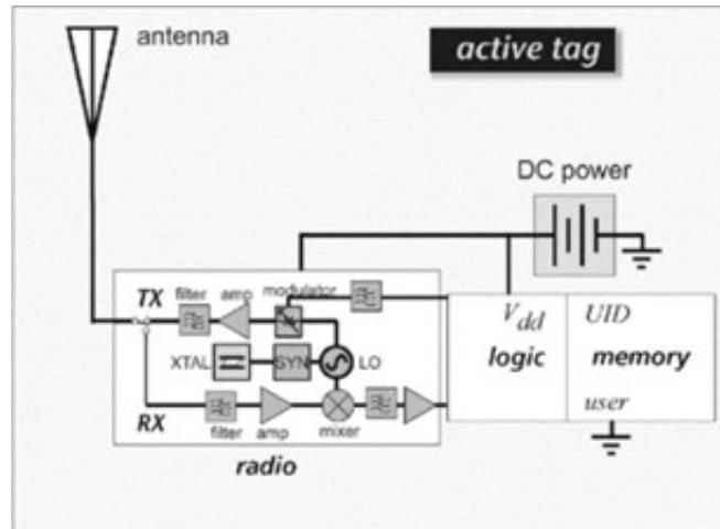
Figure 4. Active RFID Tag. Source: Dobkin (2007).
