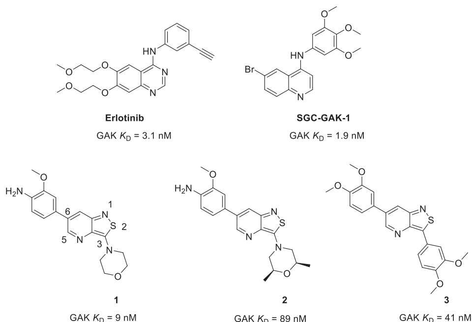
Fig. 1. Previously studied GAK inhibitors.
