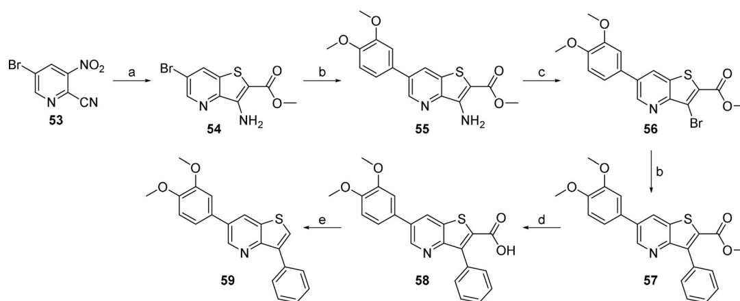
Scheme 8. Synthesis of thieno[3,2- b ]pyridine: a) ethyl 2-mercaptoacetate, KOtBu, DMF (54 %); b) 3,4-dimethoxyphenyl-B(OH) 2 (76 %) or phenyl-B(OH) 2 (42 %), K 3 PO 4 , Pd(PPh 3 ) 4 , dioxane, 110 °C; c) t BuONO, CuBr 2 , CH 3 CN (47 %); d) NaOH, EtOH, RT (89 %); e) Cu, quinoline, 200 °C (48 %).
