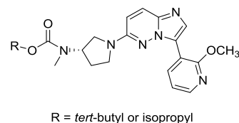
Figure 2. AAK1 inhibitors with documented antiviral activity.
