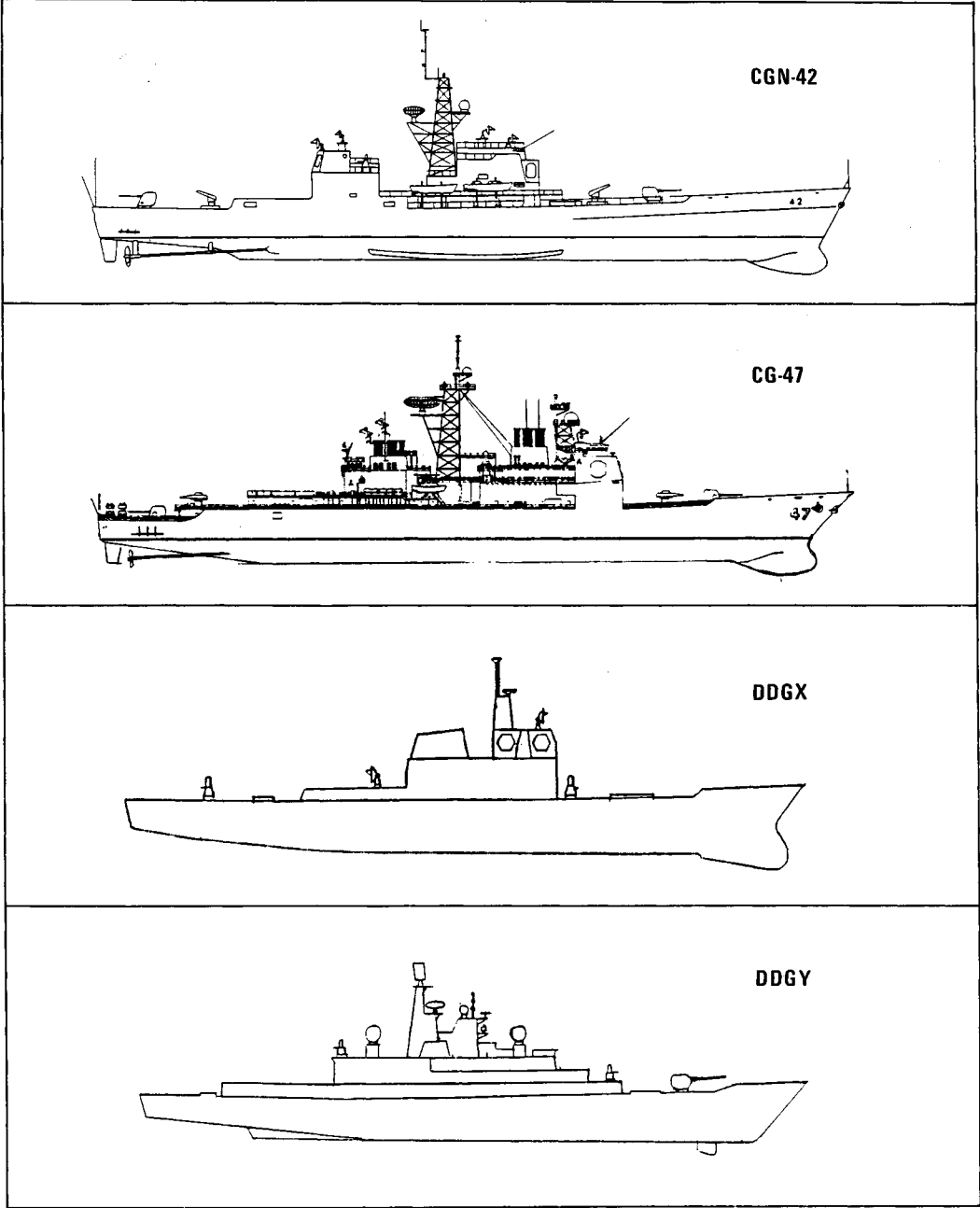
Figure E-1. Four Alternative Ship Types
