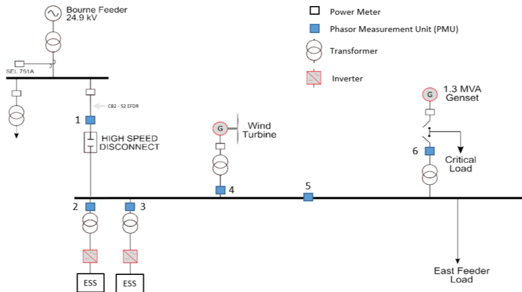
Figure 13. C-HIL Test Configuration for Testing of PXiSE ACT Controls
