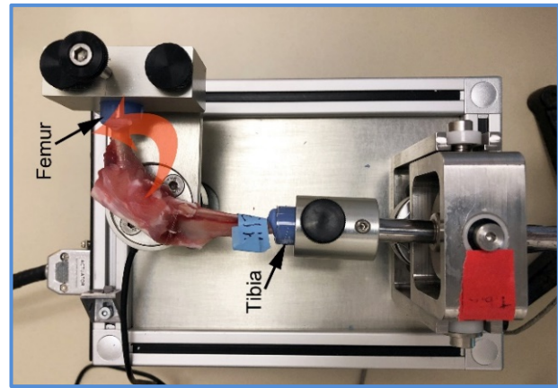
Figure 11. A depiction of a mechanical tester for measuring the joint contracture. The red arrow indicates the movement of the femur.
