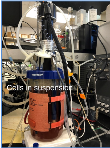
Figure 2. A new vessel of the bioreactor system we use to produce the ACA.
