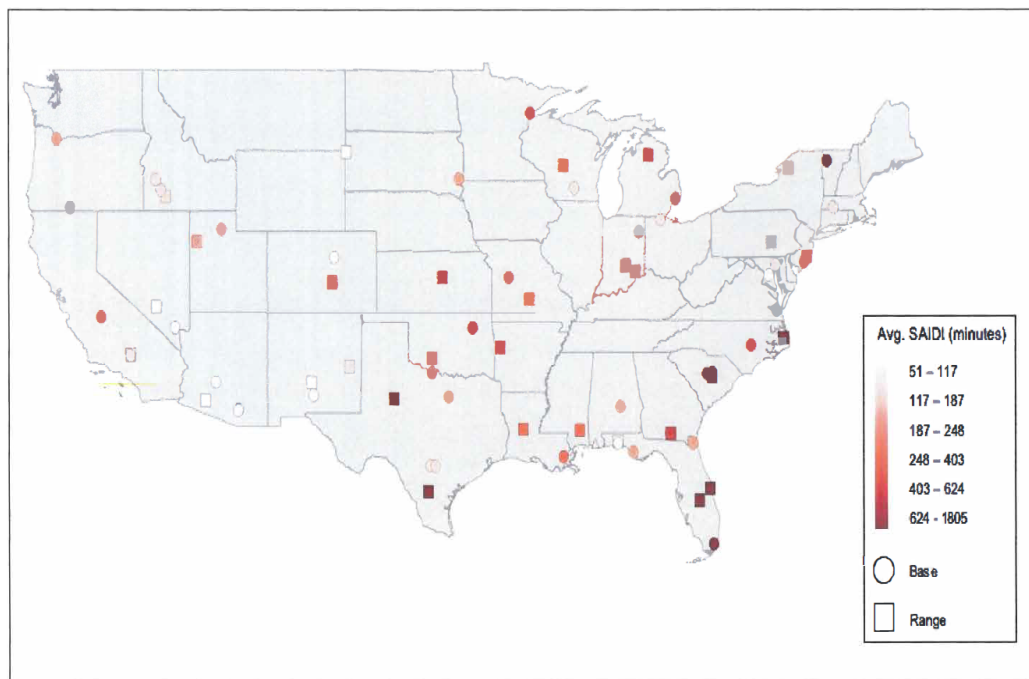
Figure 4.4. Average SAIDI Value of USAF Bases and Ranges
