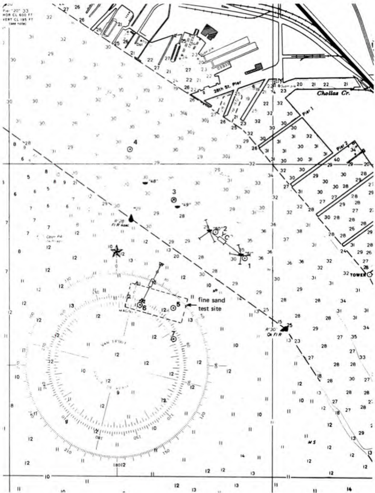
Figure 1. Test and core locations at San Diego Harbor - location 1.
