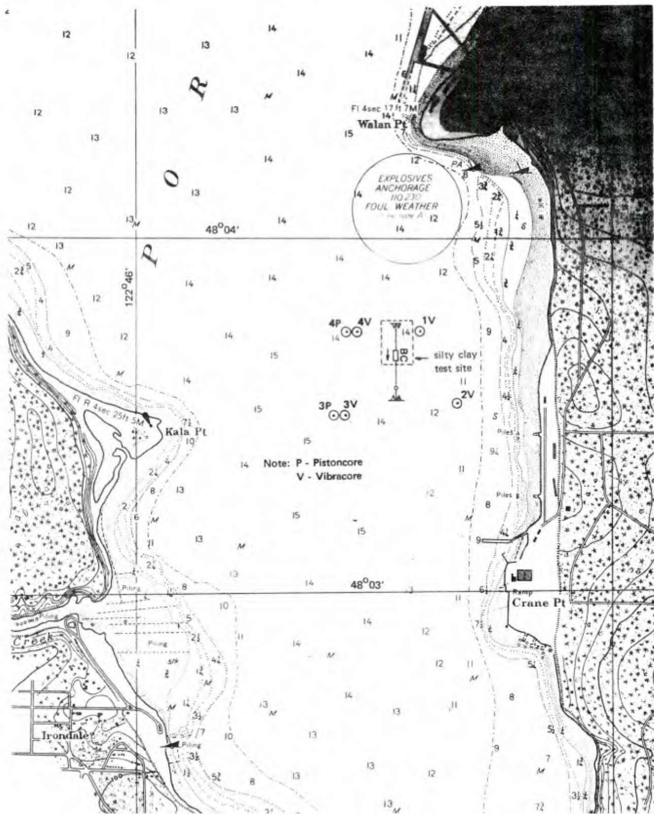
Figure 3. Test and core locations - Indian Island.
