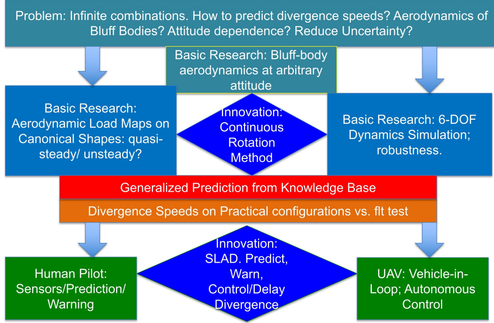
Figure 3: The transition of the Slung Loads divergence speed prediction problem, from the red of deep uncertainty and knowledge generation through basic research to the green of the SLAD implementation proposed here. The two major enabling innovations are shown in deep blue. Dynamic simulations merged the basic research through the results from the Continuous Rotation technique, and yielded the insights that bred the SLAD invention.
