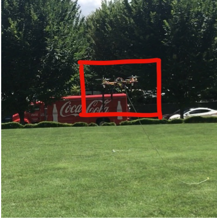
Figure 8: Single quad rotor from the scalable UAV shown during outdoor flight testing
