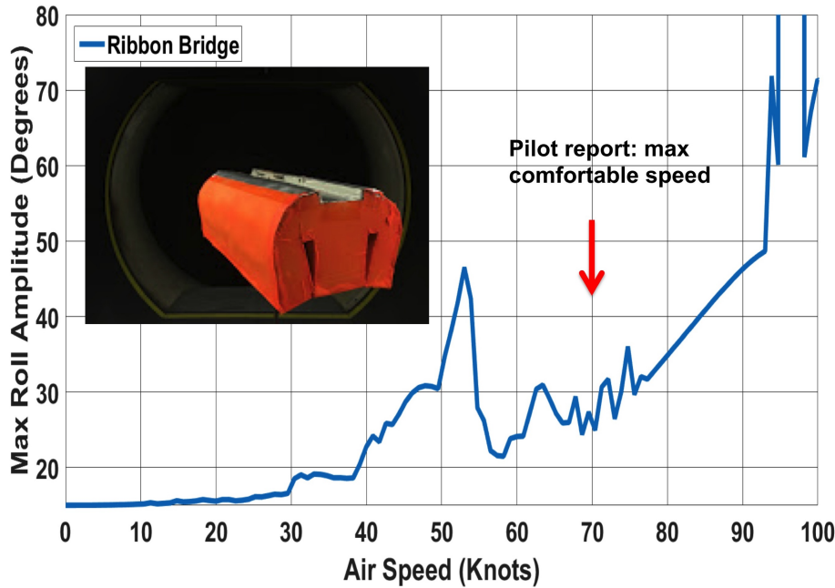
Figure 2: Maximum roll amplitude versus flight speed for a Ribbon Bridge model, predicted by dynamic simulation with model-scale wind tunnel aerodynamic data, compared to flight test points.
