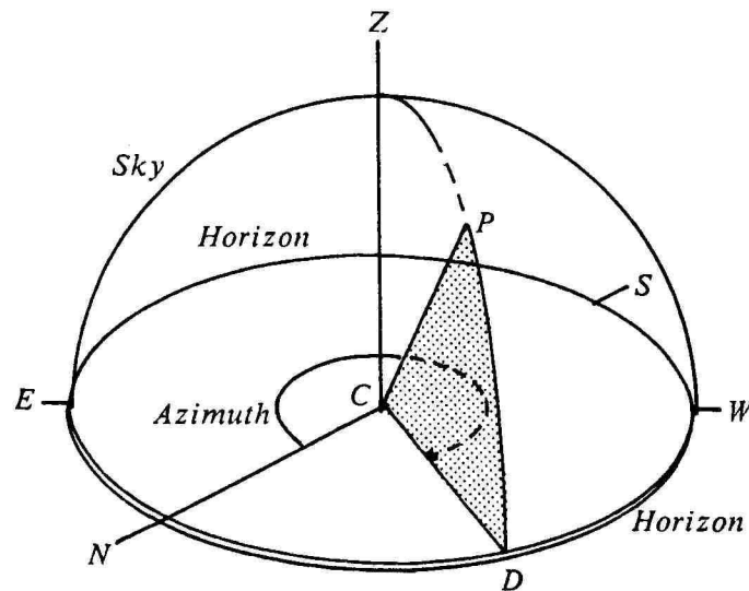
Figure 2 -- C is a point on the Earth's surface. The horizon plane, centered at C, is represented by ENDWS. The sky is shown by the arcs EZW and ZPD. The point directly overhead at C is the zenith (Z) and the direction of the vertical at C is CZ. P is the position of the Sun or Moon with direction CP as seen from C. The altitude of P is arc DP on the sky and equal to the angle between the lines CP and CD. Azimuth is the angle measured from line CN, positive eastward on the horizon plane, to line CD.
