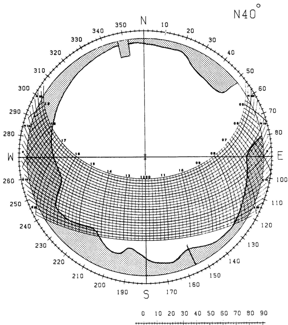
Figure 5 -- Altitude, Azimuth Diagram showing obstructed horizon.
