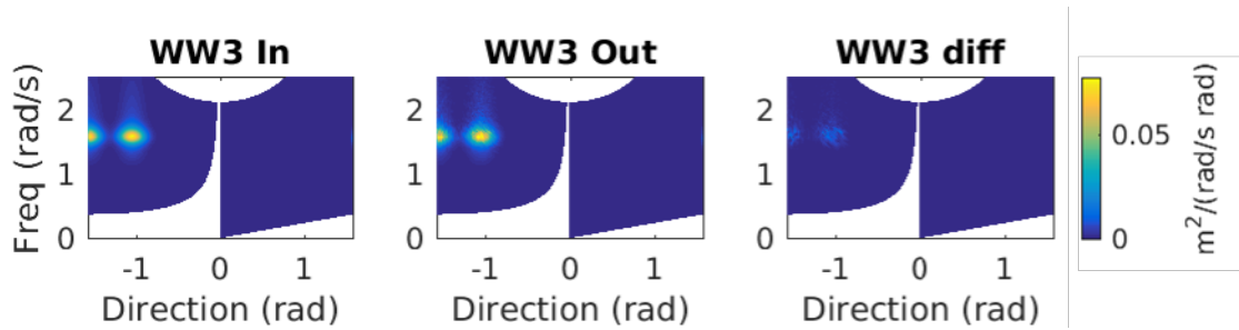
Figure 5. Beginning ( t = 1 sec, left ) and ending ( t = 100 sec, middle ) spectral states for simulation with HOS-ocean, initialized by originally symmetric bimodal spectrum shifted by ww3shift = -75^\circ . Difference between beginning and end states is shown in right panel.
