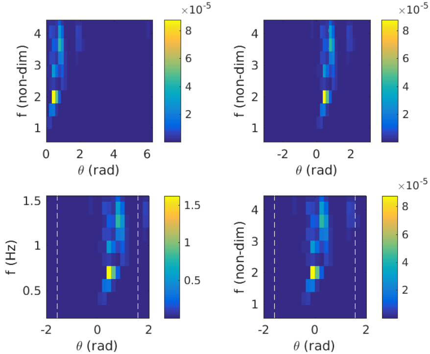
Figure 1. Spectral output of diagnostic test files generated at initiation of HOS-ocean simulation utilizing WW3 input spectrum that was shifted in direction using ww3shft = -30^\circ . Top left : ww3_unsort_dimlss.dat ; Top right : ww3_sort_dimlss.dat ; Bottom left : ww3_sorted_dimlss.dat ; Bottom right : ww3_rctr_dimlss.dat . Dashed lines in bottom two panels indicate directional limits of HOS-ocean domain, i.e., -\pi/2 < \theta < \pi/2 .
