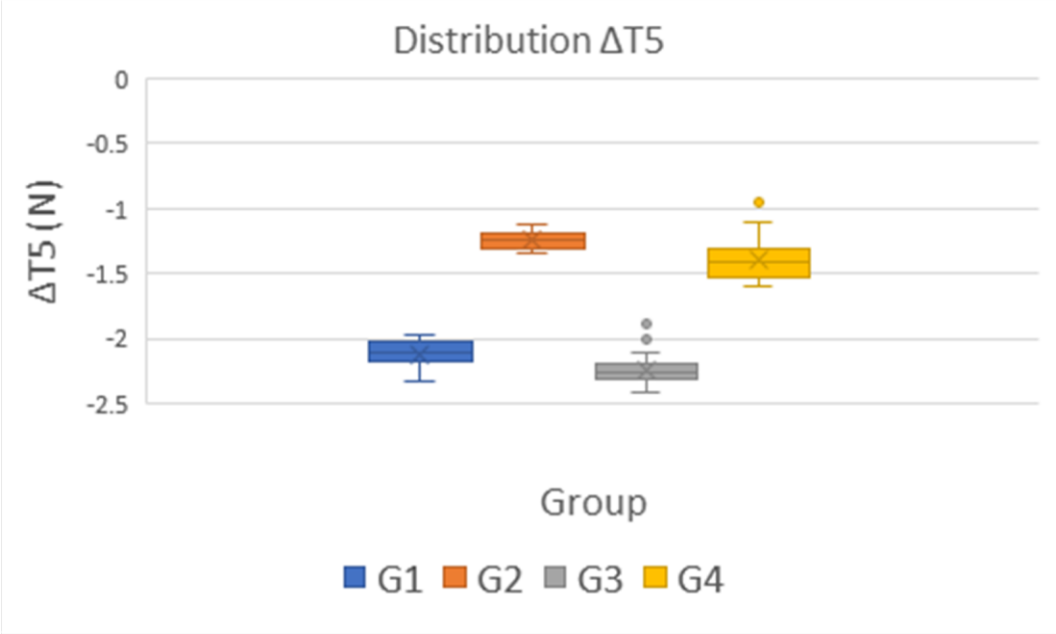
Figure VI: Force Change by Distribution
