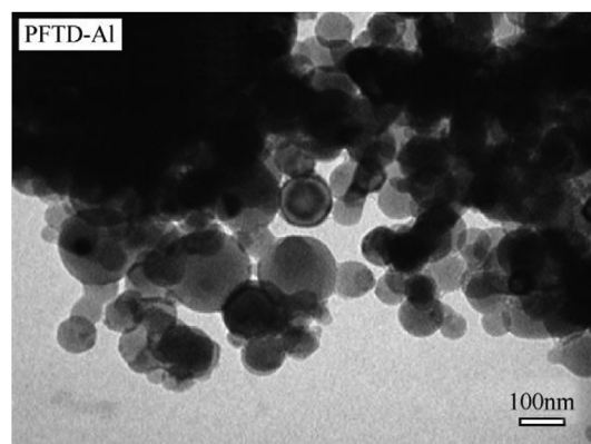
Fig. 8. TEM image of PFTD-coated bare aluminum particles [50].
