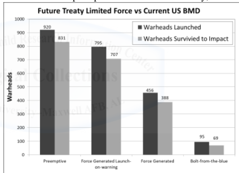
Figure 3. Results: Future treaty-limited nuclear force versus current US BMD system
