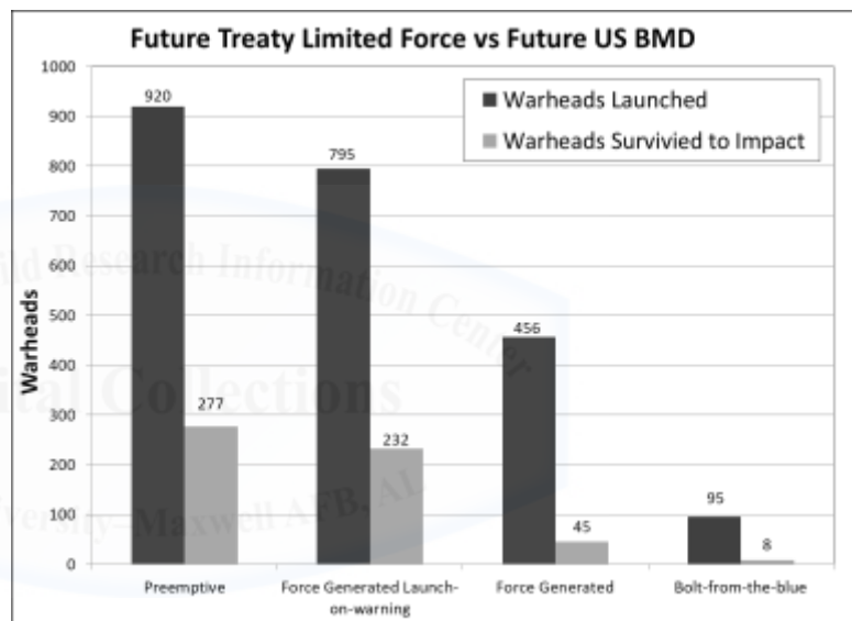
Figure 4. Results: Future treaty-limited nuclear force versus future US BMD system
