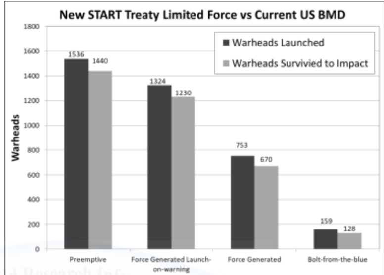
Figure 1. Results: NST-limited nuclear force versus current US BMD system
