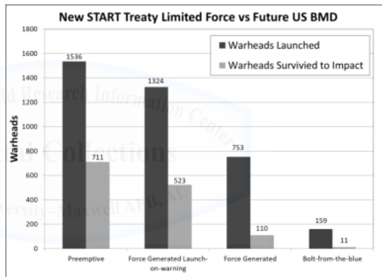
Figure 2. Results: NST-limited nuclear force versus future US BMD system
