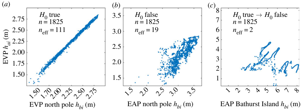
Figure 3. Demonstration of the Two-Stage Paired Thickness Test (2SPT) for daily concentration-weighted ice thickness series from the Regional Arctic System Model (RASM) extending for 5 years from 1996 to 2000 ( n = 1825 ): (a) The Stage-1 t -test in equation (3.3) confirms the null hypothesis, H_0 : \mu_{\Delta} = 0 , for h_{ai} and h_{bi} taken from adjacent grid cells at the North Pole for the EVP simulation. (b) The t -test in equation (3.3) confirms the alternate hypothesis, H_1 : \mu_{\Delta} \neq 0 , for respective h_{ai} and h_{bi} series co-located at the North Pole for EVP and EAP simulations, so that the test stops at Stage-1 even though n_{\text{eff}} < 30 . (c) The test proceeds to Stage 2 because n_{\text{eff}} < 30 for co-located perennial ice time series north of Bathurst Island and the t -test in equation (3.3) confirms H_0 . The Stage-2 test using equation (3.1) with the look-up table in table 2 subsequently corrects the outcome to confirm the alternate hypothesis, H_1 . Time series locations used in this figure are tagged in figure 4 h in magenta. (Online version in colour.)
