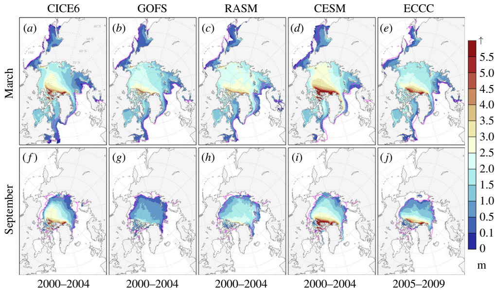
Figure 1. (a–e) March and (f–j) September Arctic mean 0000 UTC sea-ice thickness from five models summarized in table 1 for years 2000–2004 except for ECCC, which are for 2005–2009. CESM large ensemble averages are constructed from the first five ensemble members. Thicknesses are plotted only for model sea-ice concentrations greater than 15%. Magenta contours indicate observed mean March and September sea-ice extent calculated from the NOAA/NSIDC Climate Data Record [25].
