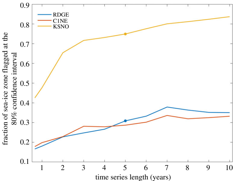
Figure 5. Fraction of the Northern Hemisphere CICE6 grid points with h_{ai} > 0.01 m or h_{bi} > 0.01 m for which the alternate hypothesis H_1 is true at the point of Categorization in the 2SPT test and as a function of run length after model initialization on 1 January 2000. The graph is constructed from daily h_{ai} and h_{bi} values at each grid point analysed up to n = 240, 365, 730, 1095, 1460, 1825, 2190, 2555, 2920, 3285 and 3650 for each of the RDGE, CINE and KSNO simulations, respectively. Blue (RDGE) and red (CINE) traces indicate results for code changes that are neither bit-for-bit nor climate altering, whereas the yellow (KSNO) trace is the result of a tiny climate-modifying parameter change in the model. Round markers on the RDGE and KSNO traces correspond to the flagged regions mapped in figure 4e,f at n = 1825 .
