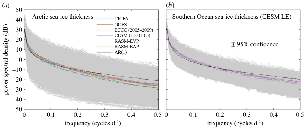
Figure 2. Power spectral density of perennial concentration-weighted sea-ice thickness h_i (a) for the Arctic for all models and (b) for the Southern Hemisphere from the CESM Large Ensemble. Spectra of individual model grid cells are displayed in grey, and the mean of each simulation's spectra appear in colour, including individual traces for CESM ensemble members 01 to 05. All spectra represent the period 2000–2004 (except for ECCC, 2005–2009). The GOFs spectral mean has been obtained by sampling one model cell per each 10 \times 10 grid point mat due to the resolution of that model. RASM spectra are shown for two rheological configurations: EVP as in figure 1, and EAP, corresponding to previously published results [21,22]. Converged Monte Carlo AR(1) spectral estimates appear in black, and the confidence interval displayed in (b) also applies to (a). The limited spread of spectra for the Southern Ocean relative to the Arctic is due to the comparatively small area of perennial ice that occurs in the Southern Hemisphere.
