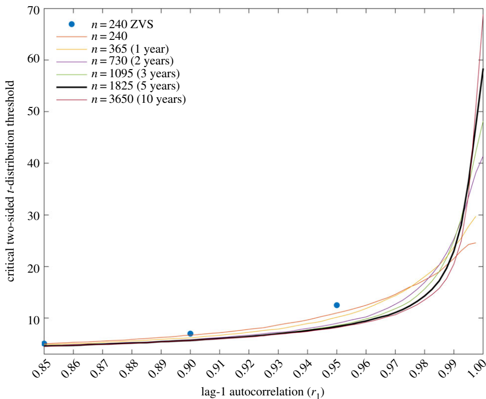
Figure 7. Critical t -statistics at the high end of the r_1 scale for the 80% two-sided confidence interval generated using the method described in the appendix. Change in the statistic with increasing sample sizes is indicated for the maximum sample size explored by Zwiers and von Storch (ZVS) in [39], n = 240 , out to the equivalent of a 10-year series of daily thickness samples from sea ice models, n = 3650 (no-leap calendar). Tabulated values from Zwiers & von Storch [39] appear as blue data points and are comparable with the n = 240 red trace generated using the large ensemble method used in this paper. The statistic for the baseline series length used by the CICE Consortium, n = 1825 , appears in bold black.
