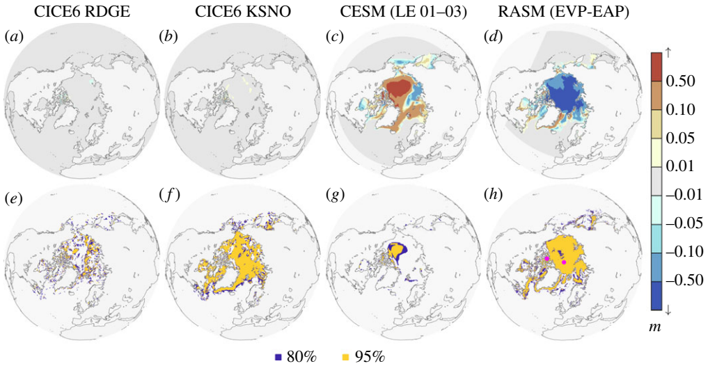
Figure 4. 2000–2004 mean 0000 UTC daily sea-ice thickness difference \bar{h}_\Delta for the (a) RDGE and (b) KSNO simulations when compared with the baseline CICE6 simulation, while (c) compares CESM Large Ensemble members 01 and 03, and (d) provides the RASM EVP minus EAP comparison. (e–h) Flag regions for which the alternate hypothesis H_1: \mu_\Delta \neq 0 is true after Stage 2 of the 2SPT test at the 80% (blue) and 95% (amber) two-sided confidence intervals. Magenta markers in (h) indicate the location of the North Pole and Bathurst Island coastal time series in figure 3. Grey shading in (a–d) indicates the extent of the analysed domain for each respective model.
