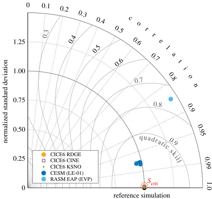
Figure 6. Taylor diagram illustrating the weighted quadratic skill score ( S ) for cases RDGE, C1NE and KSNO in the 2SPT Test shown in figures 4 and 5, compared with the reference simulations shown in figure 1. The critical quadratic skill score contour, S_{\text{crit}} = 0.999 , is illustrated in red. The standard deviation is normalized against the relevant reference simulation (black) with perfect correlation. CICE6 RDGE, C1NE and KSNO markers appear in virtually the same location within the critical threshold, referenced against the CICE6 control, and the reference simulations for CESM and RASM cases are indicated in parentheses within the legend.
