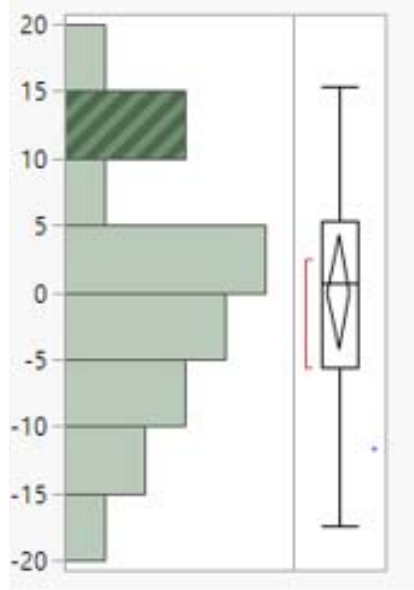
Figure 8. Residual Distribution Histogram
