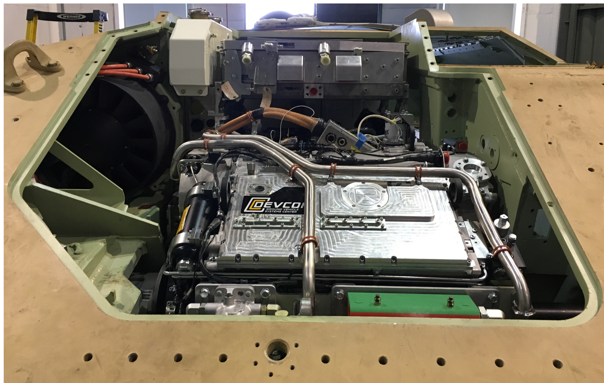
Advanced Thermal Management System
