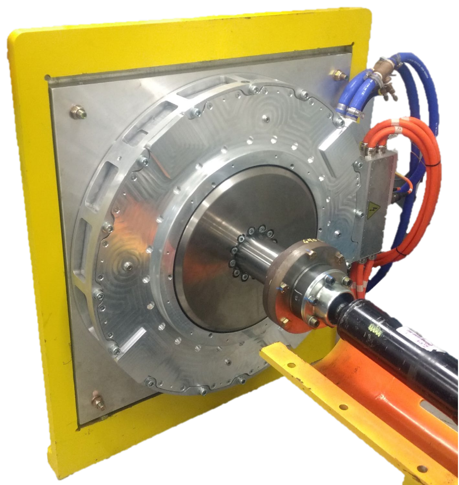
Integrated Starter Generator
