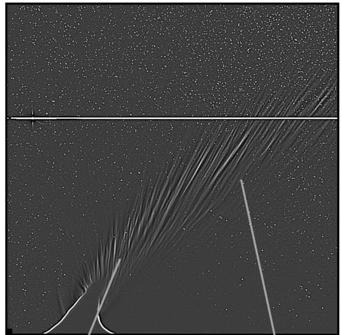
Fig. 16. The tail of McNaught on 2007 January 15 at 02:01 UT, as captured by HI-1 on STEREO-A, enhanced by subtracting a gaussian blurred version of the frame. The two insets show the clear difference between (a) the “interleaved” striae towards the south (left) part of the image, and (b) a region where striae remain largely near-parallel towards the north. The progression from near-aligned to interleaved spreads across the whole tail over time, as the comet moves towards the south.
