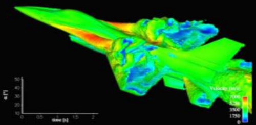
Pitching F-16 (DES SARC) \Omega iso-surface
