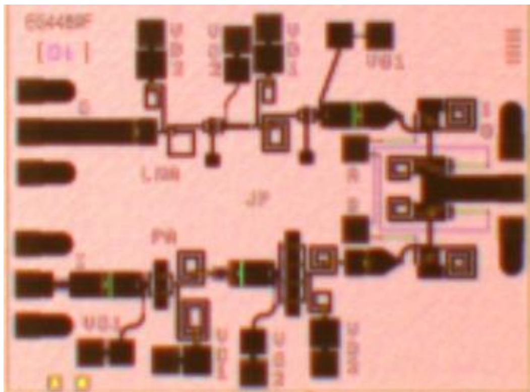
Fig. 25 Die photo of T/R Module 1: SPDT–SS, PA, and LNA
