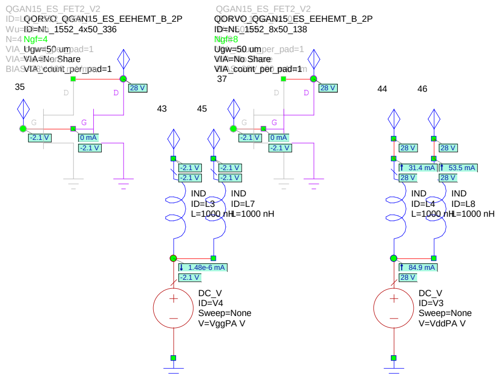
Fig. 44 DC annotation of PA HEMTs verifying bias of physical layout for TRS 3 (28 V; 150 mA/mm)
