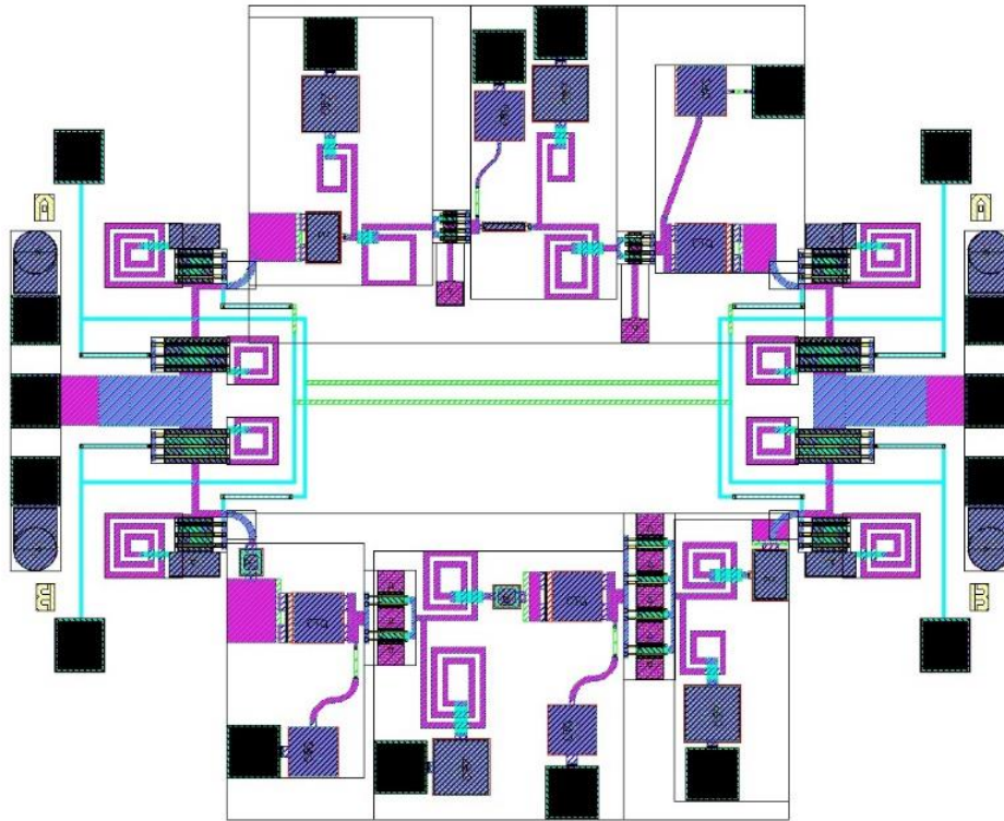
Fig. 40 Layout plot of T/R Module 3: LNA at top, PA at bottom (2 mm × 1.5 mm)
