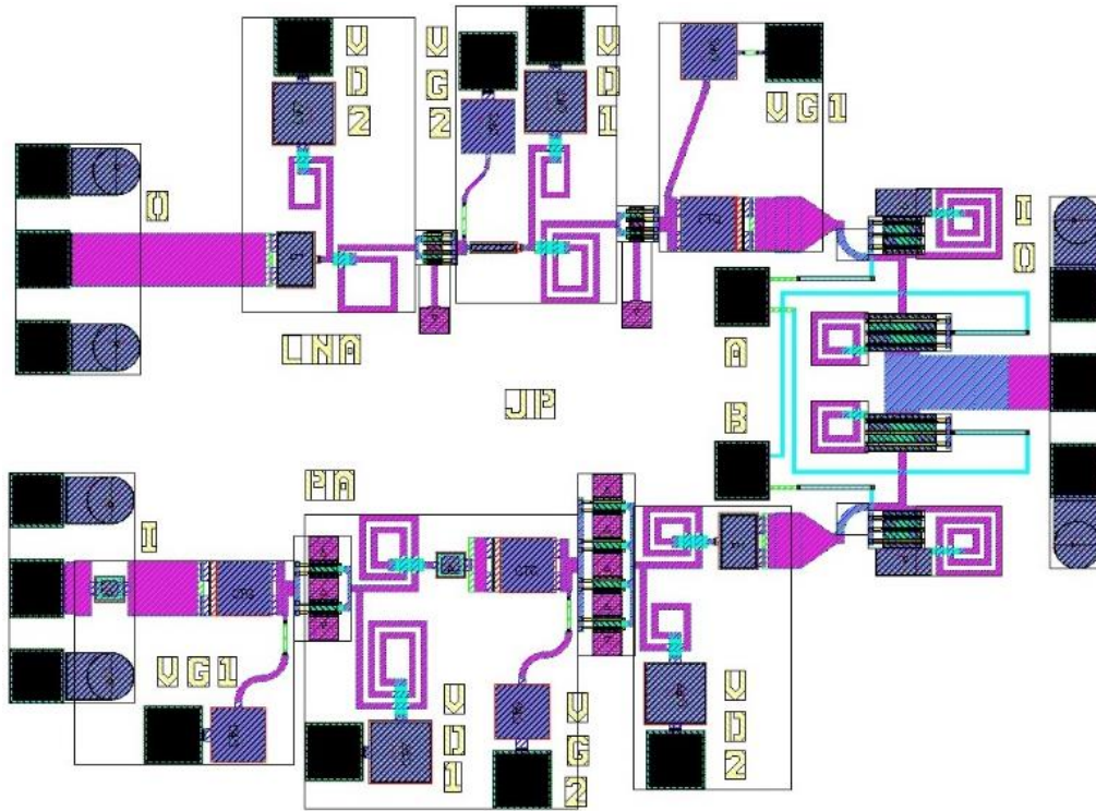
Fig. 54 Layout plot of T/R Module 1: LNA at top, PA at bottom (2 mm × 1.5 mm)
