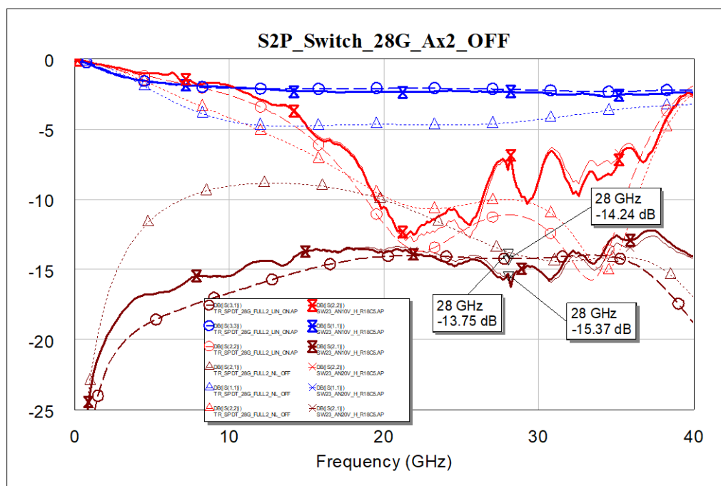
Fig. 24 Measured (solid) vs. simulation (dash) T/R Switch no. 2 “OFF”
