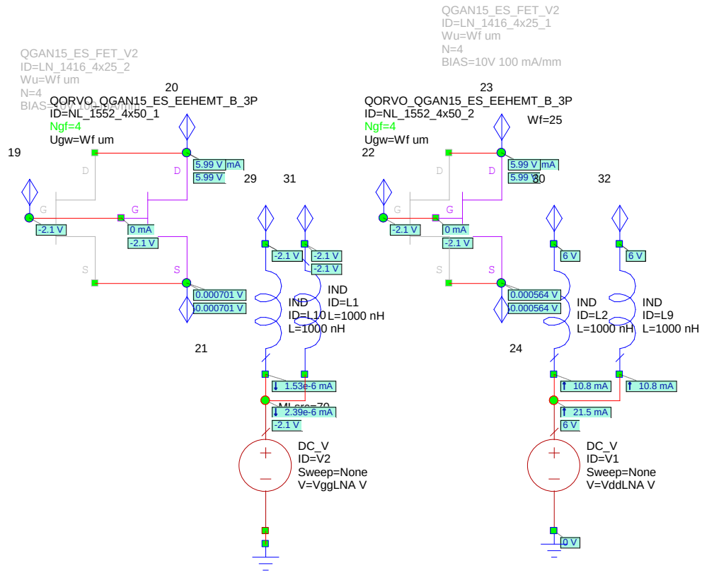
Fig. 51 DC annotation of LNA HEMTs verifying bias of physical layout for TRS 2 (6 V; 100 mA/mm)
