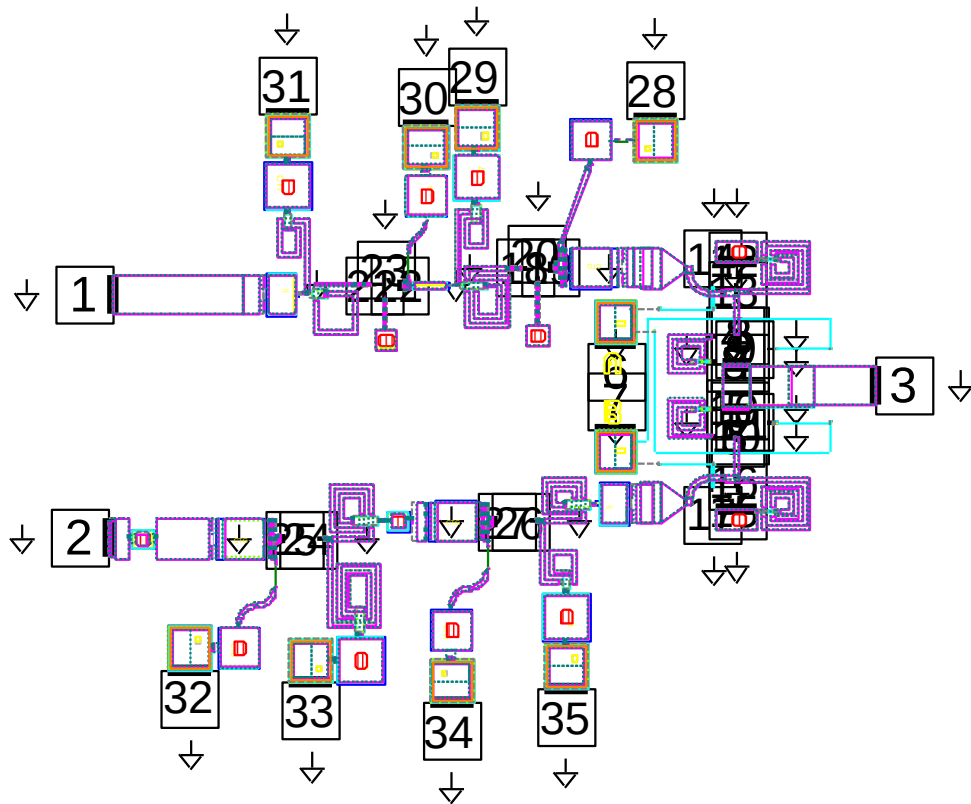
Fig. 55 2-D Axiem EM plot of T/R Module 1 (35 ports)
