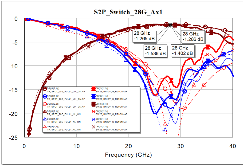
Fig. 21 Measured (solid) vs. simulation (dash) T/R Switch no. 1 “ON”
