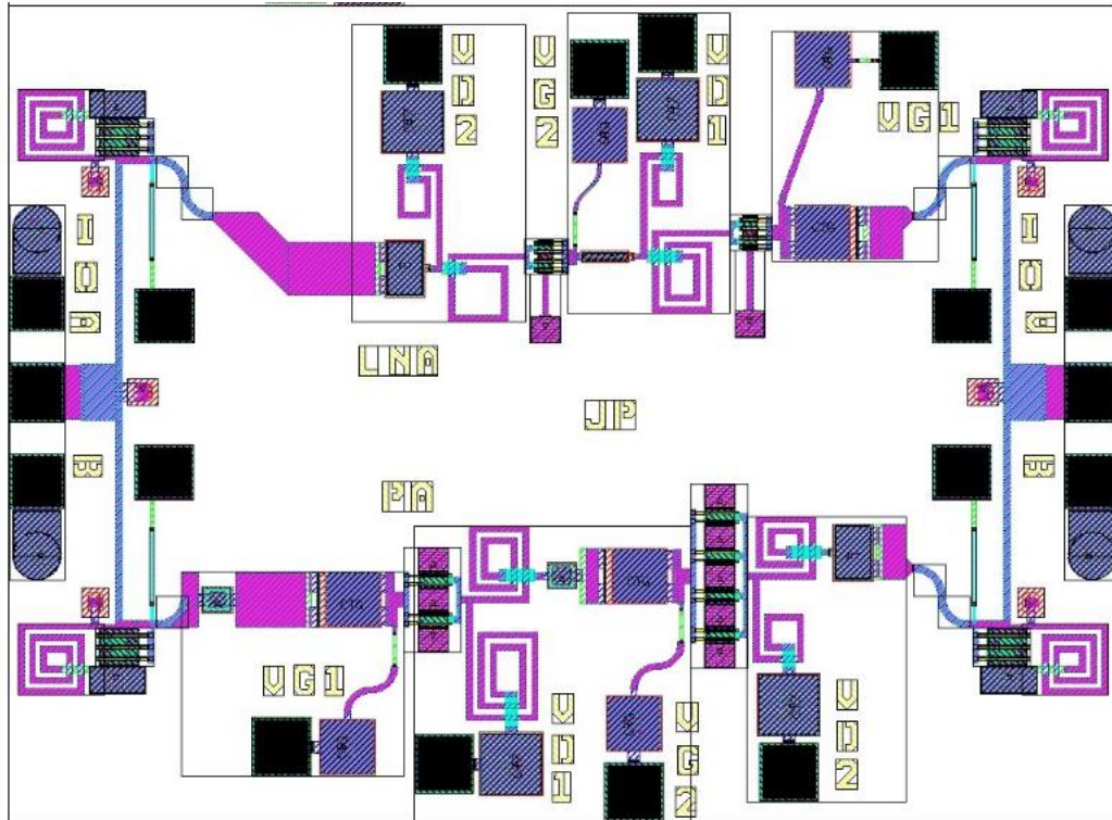
Fig. 47 Layout plot of T/R Module 2: LNA at top, PA at bottom (2 mm × 1.5 mm)
