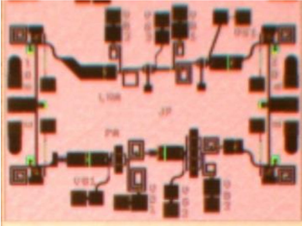
Fig. 26 Die photo of T/R Module 2: two SPDT-SO's, PA, and LNA
