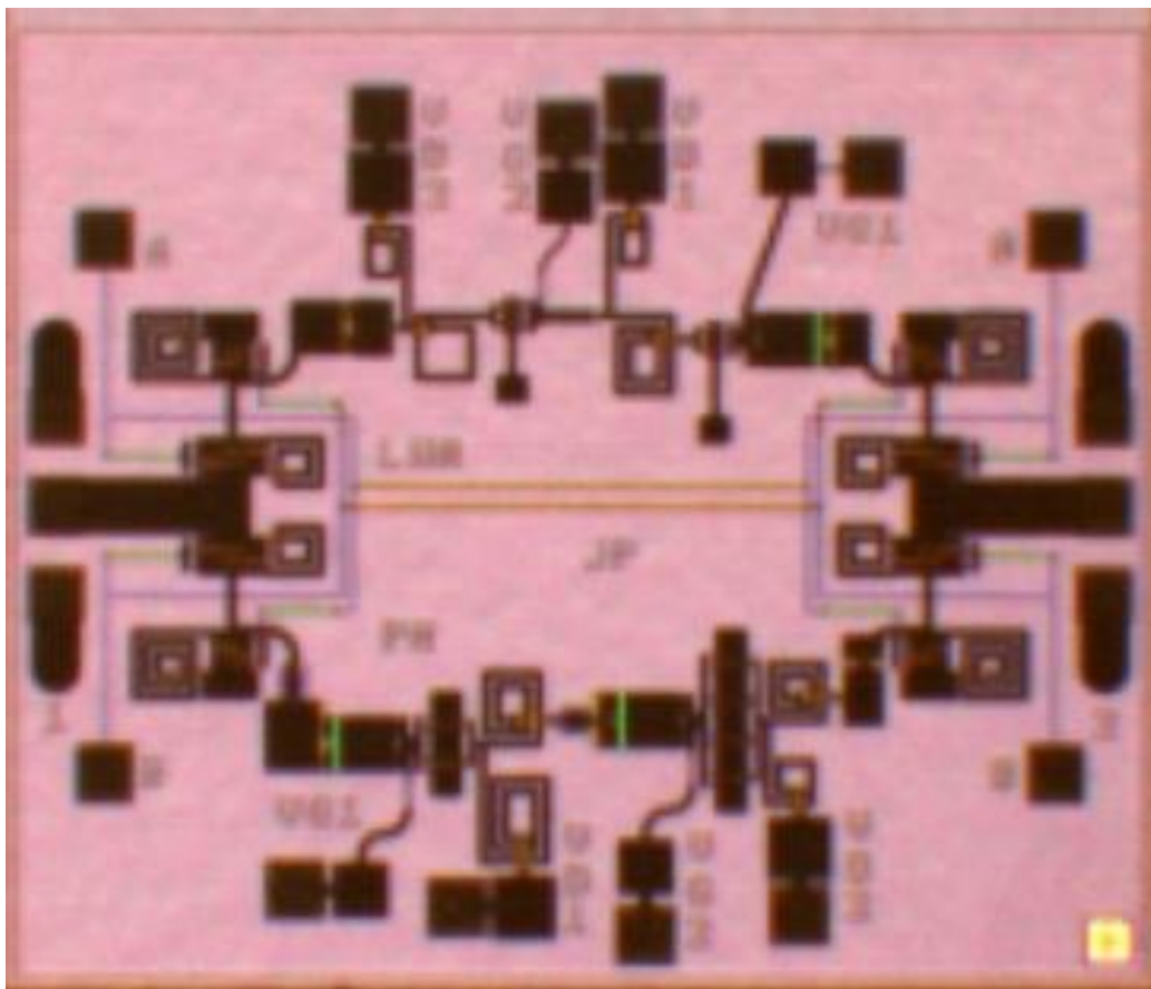
Fig. 27 Die photo of T/R Module 3: two SPDT-SS's, PA, and LNA
