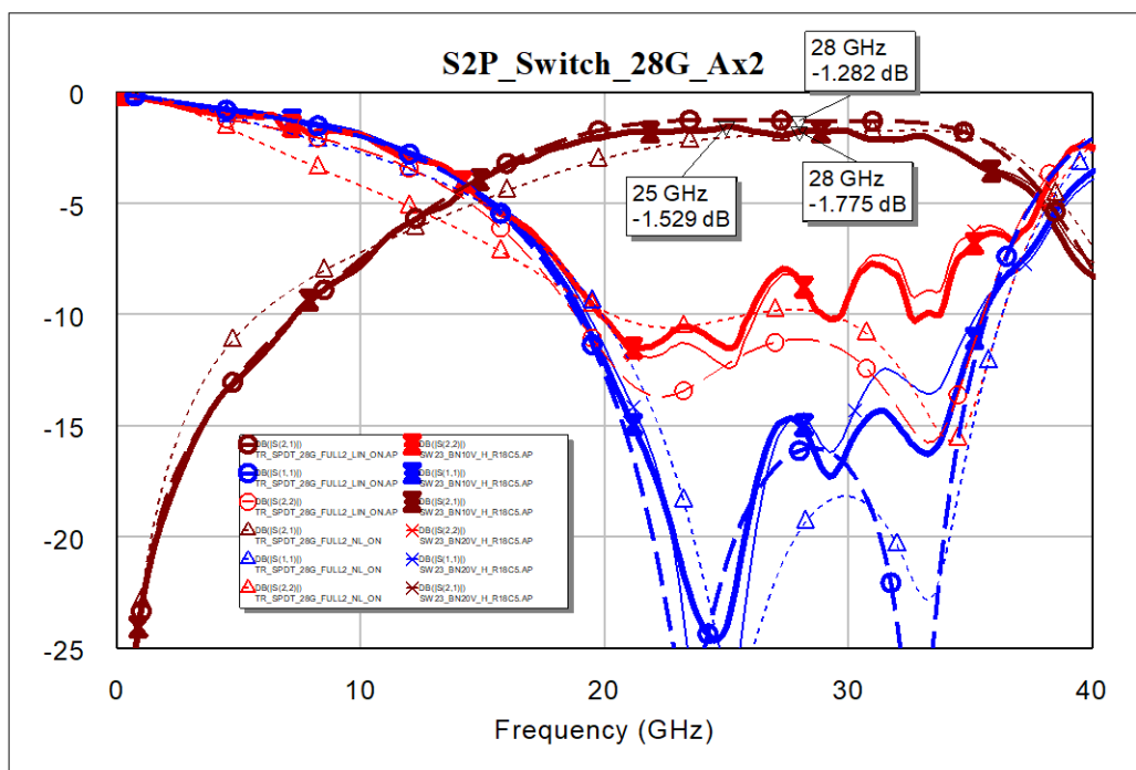
Fig. 23 Measured (solid) vs. simulation (dash) T/R Switch no. 2 “ON”
