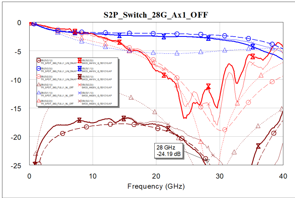
Fig. 22 Measured (solid) vs. simulation (dash) T/R Switch no. 1 “OFF”
