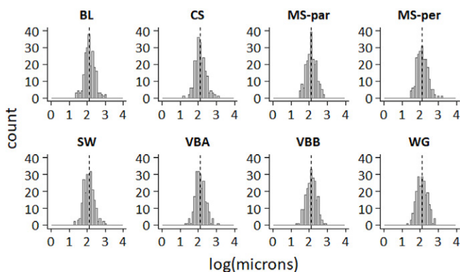
Fig. 3. Log-transformed frequency distributions for the individual measurements of the aperture width of the visible fracture, x , pooled for each rock type: Burlington Limestone (BL), Crossville Sandstone (CS), Mancos Shale, cored both parallel (MS-par) and perpendicular (MS-per) to bedding, Sierra White Granite (SW), Vermilion Bay Granite A (VBA), Vermilion Bay Granite B (VBB), and Westerly Granite (WG).
