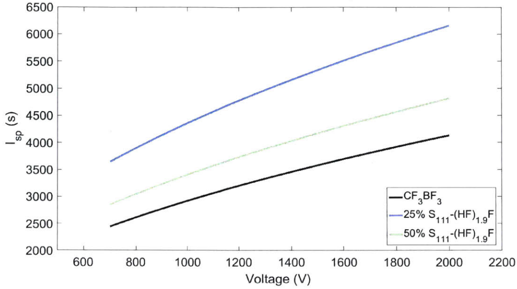
Figure 2-13: I_{sp} bounds for FHIL mixtures.
