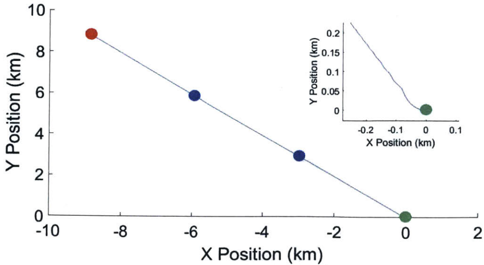
Figure A-17: Trajectory of WaferSat with 0.1° thrust vector offset.
