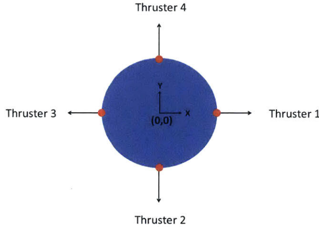
Figure A-6: WaferSat with purely radial thrusters.
