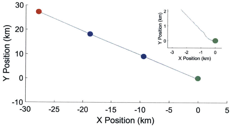
Figure A-16: Trajectory of WaferSat with 0.01° thrust vector offset
