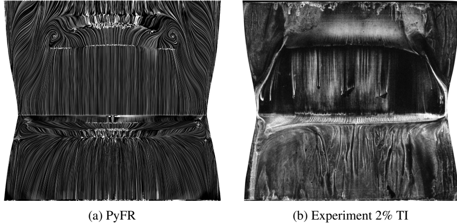
Figure 23. Image of computational shear LIC lines (a) and experimental oil-streak lines (b) on the pressure and suction sides of the LPT blade surface.
