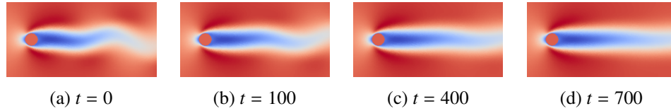
Figure 25. Snapshots of x -momentum over time as the MPC algorithm attempts to suppress vortex shedding.
