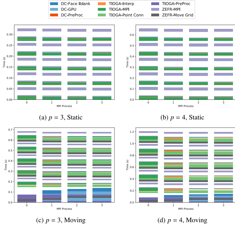
Figure 9. Timeline of overset grid work during one full five-stage explicit time step over all ranks of the Taylor Green test case. Top: Static overset grids; Bottom: Moving overset grids. The prefix ‘DC’ refers to work specific to our Direct Cut method; ‘TG’ refers to standard procedures used within TIOGA; and ‘ZEFR’ refers to work performed within the solver.
