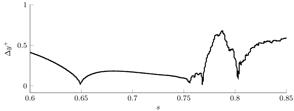
Figure 21. Distribution of \Delta y^+ along the suction side of the blade.
