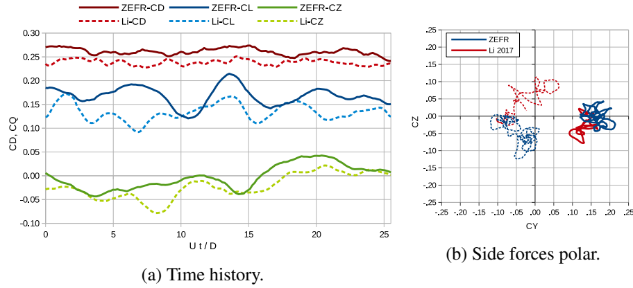
Figure 5. Comparison of force time histories for our spinning golf ball vs. the results from Li et al. 2017. The dashed curves in (b) re-plot the same polar data from the static golf ball cases.
