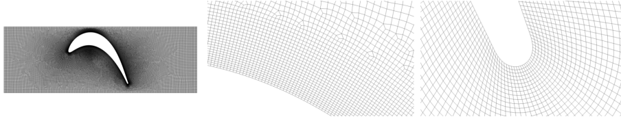
Figure 20. Two dimensional cross-section of the hexahedral mesh used for the T161 simulations.
