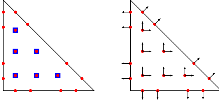
Figure 16. Degrees of freedom on reference triangle for P = 2 . The solution points are represented by blue squares, flux points are represented by red circles, and unit vectors for Raviart–Thomas flux interpolation are represented by black arrows.
