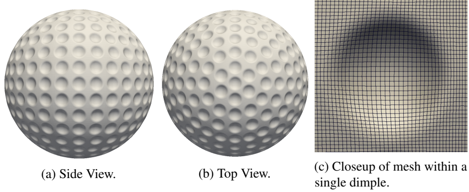
Figure 2. Golf ball surface. Figure (c) shows the pre-agglomerated element sizes; the actual surface resolution of the golf ball is 4/3 times greater than that shown.
