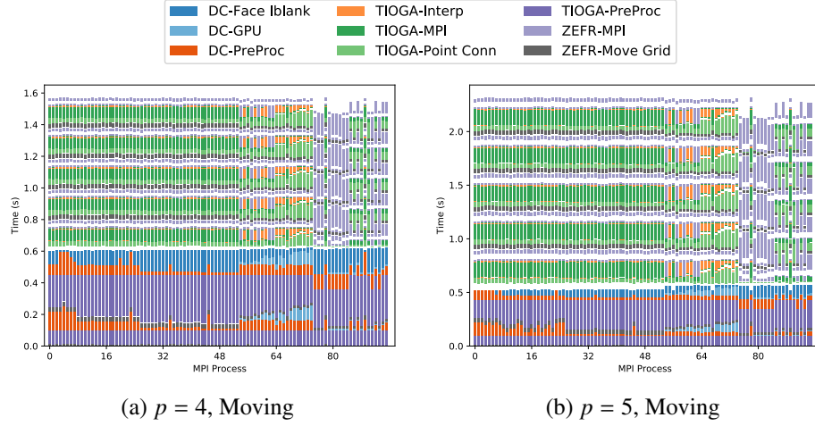
Figure 13. Timeline of overset operations for the golf ball case across 96 GPUs.
