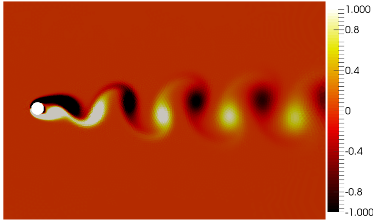
Figure 18. Vorticity contours of cylinder at Re = 100 , range scaled to [-1, 1] for emphasis
