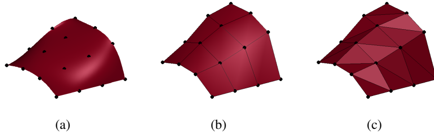
Figure 1. Example of splitting a high-order quadrilateral into linear triangles. (a) The exact tensor-product Lagrange polynomial representation; (b) Treating the tensor-product grid as a grid of linear quadrilaterals; (c) Splitting linear quads into triangles.
