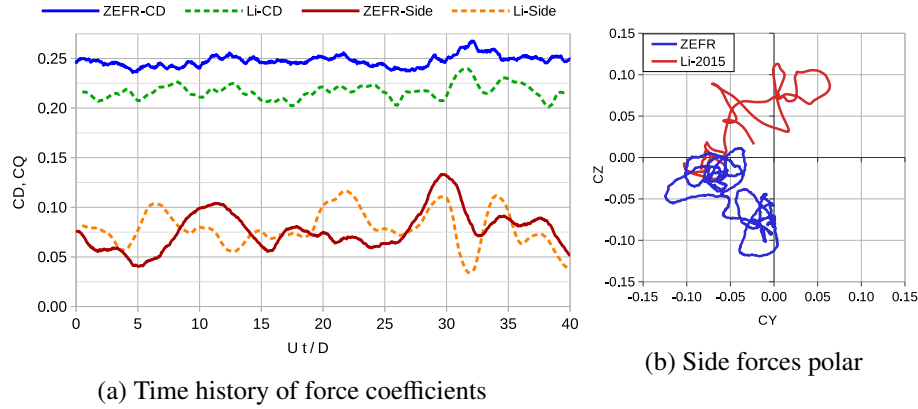
Figure 4. Force coefficients for the static golf ball simulation, compared with those produced by Li et al. under similar conditions.
