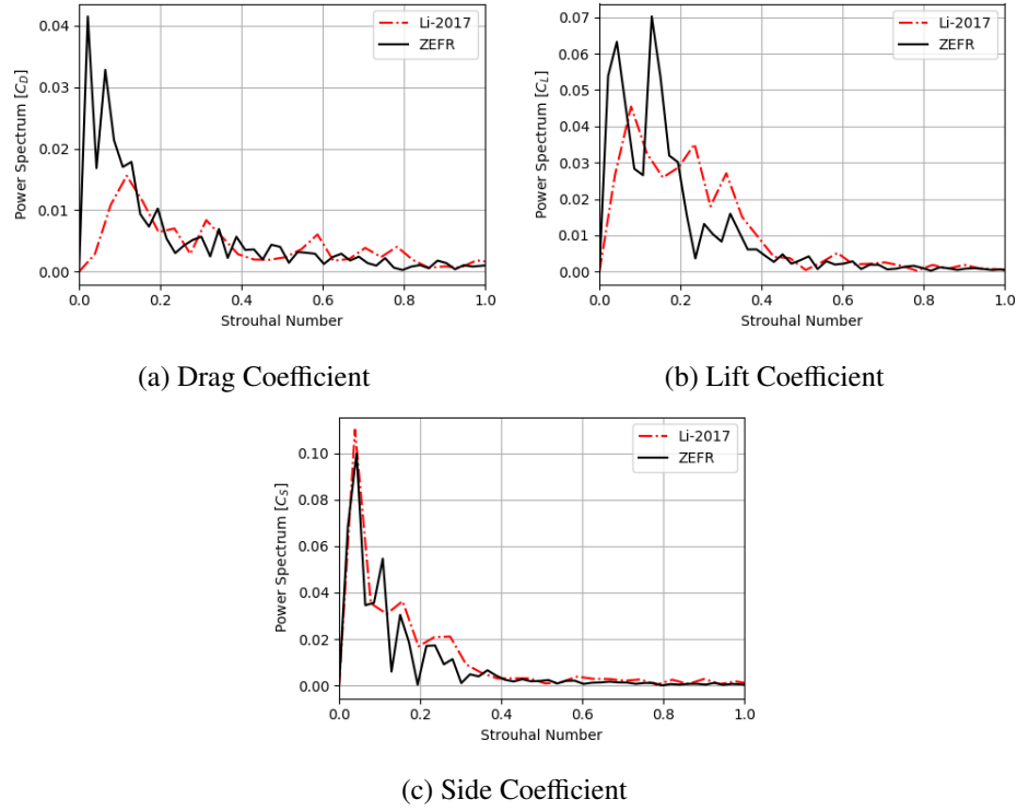
Figure 6. Comparisons of power spectrum density for our spinning golf ball vs. the results from Li et al. 2017
