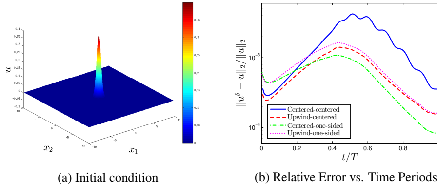
Figure 15. Initial condition and relative error of the propagation of an approximate Gaussian. The advection-diffusion equation is solved using the FR method.
