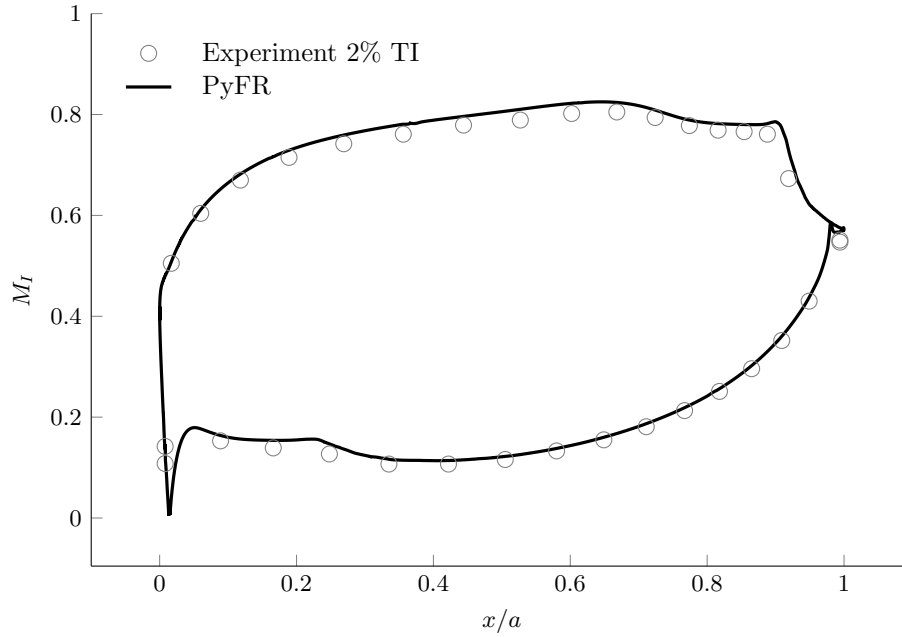
Figure 22. Distribution of M_I over the pressure and suction sides of the LPT blade surface at mid-span.
