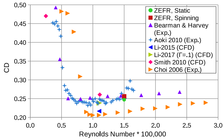
Figure 8. Comparison of C_D values from several experimental and computational studies.
