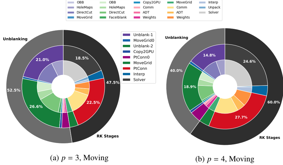
Figure 12. Breakdown of time spent on overset-related tasks for moving grids on GPUs (3-node, 48-GPU golf ball case). Middle layer: High-level overset tasks; Inner layer: Lower-level subtasks for each slice of the middle layer.
