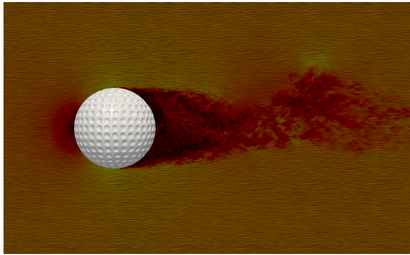
Figure 3. View of approximate streamlines and velocity magnitude field through the y = 0 plane (golf ball centerline).
