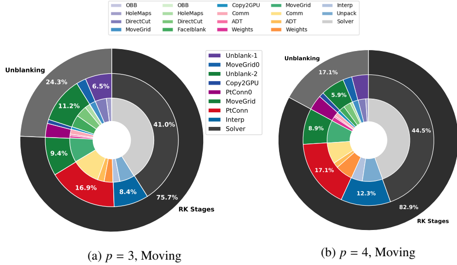
Figure 10. Breakdown of time spent on overset-related tasks for moving grids on GPUs (single node, 4-GPU case). Middle layer: High-level overset tasks; Inner layer: Lower-level subtasks for each slice of the middle layer.
