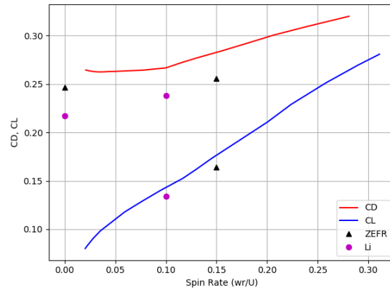
Figure 7. C_D and C_L vs. nondimensional spin rate. Data for conventional golf balls over a wide range of supercritical Reynolds numbers, from Figure 9 of Bearman and Harvey [3]
