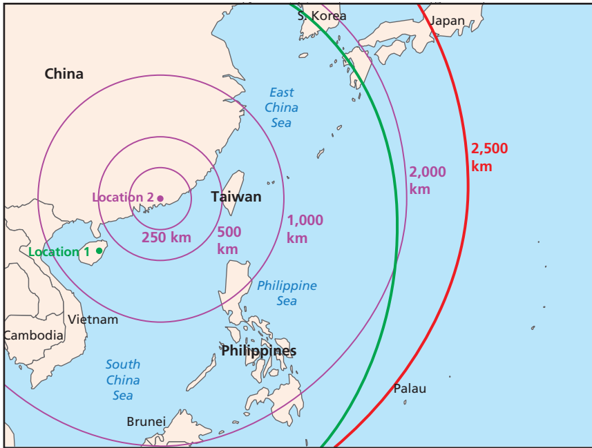
Figure 6.5 Ranges from the Chinese Mainland to the Philippines
