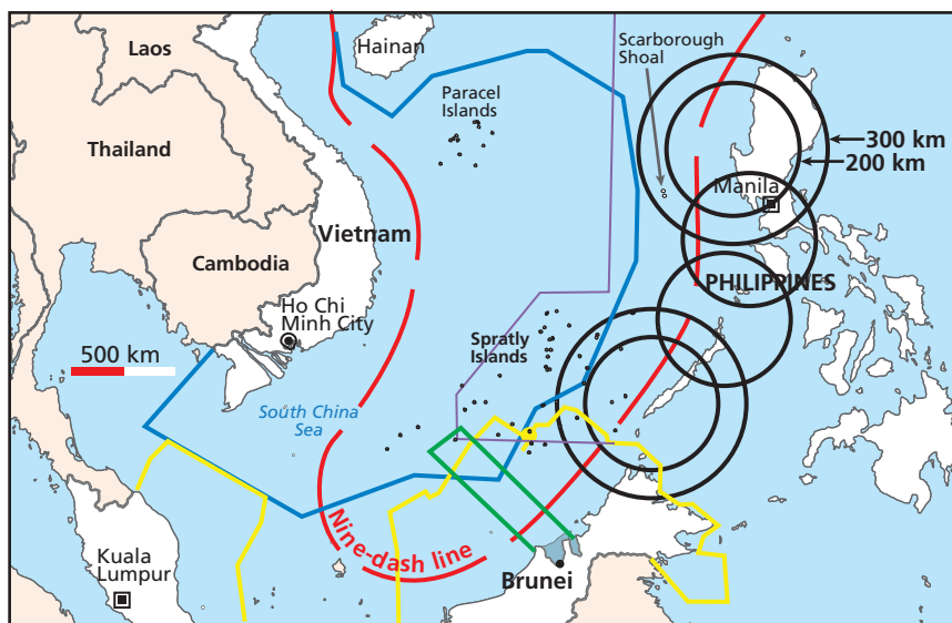
Figure 6.6 Coverage of the South China Sea from the Philippines
