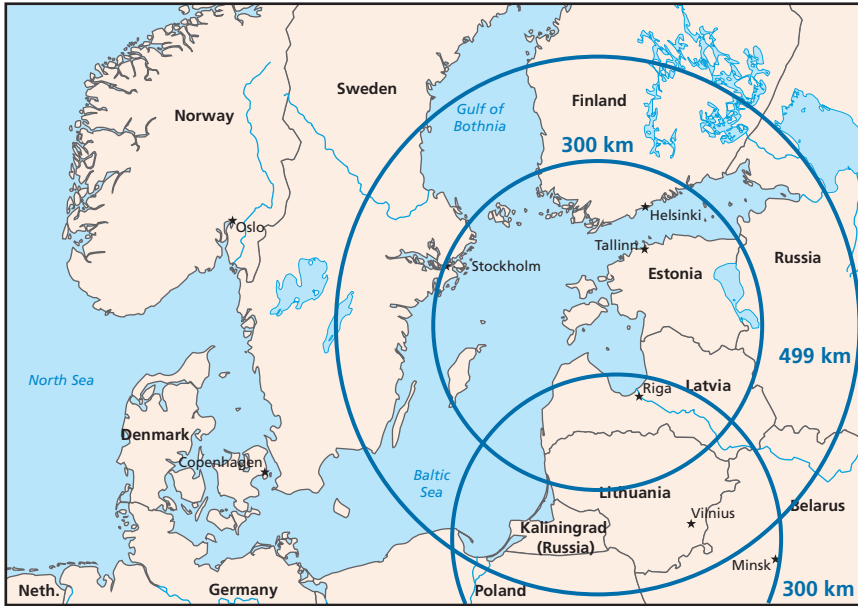
Figure 6.9 Coverage of the Baltics, Belarus, and Russia from Poland and Estonian Coastal Islands
