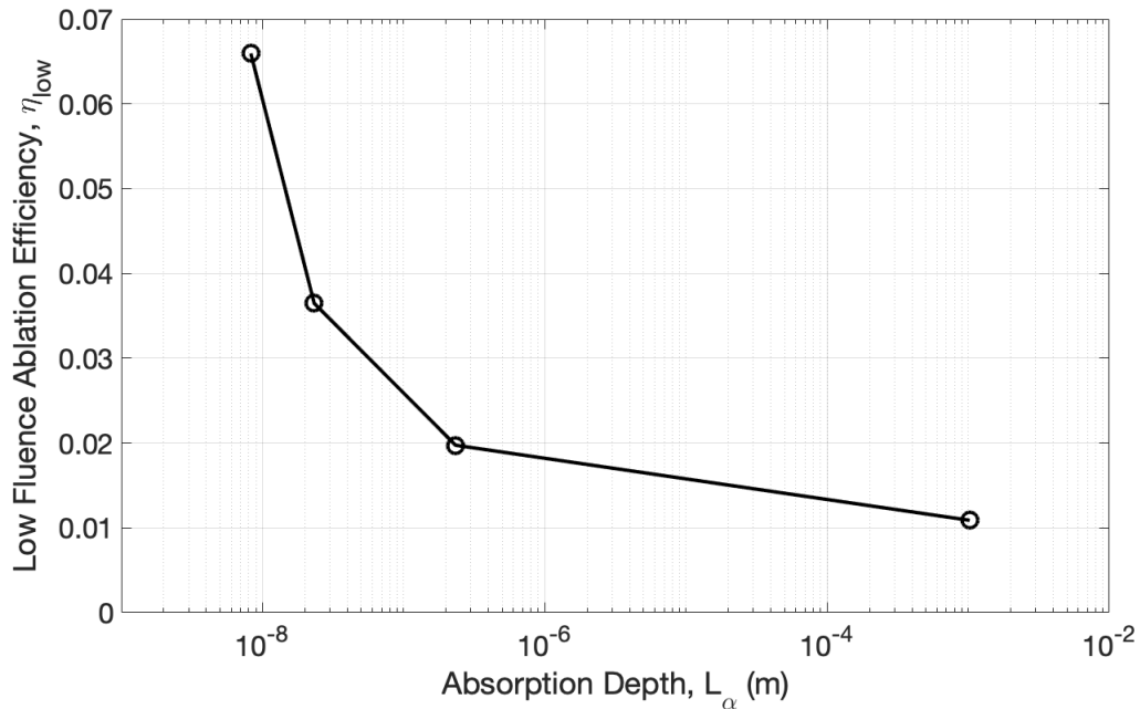
Figure 36. Low fluence ablation efficiency versus optical absorption depth. \lambda = 1064 nm, \tau_p = 28 \mu s, \omega_0 \approx 6.7 \mu m, F : varied, Material: varied, P = 1 atm, T = 300 K.
