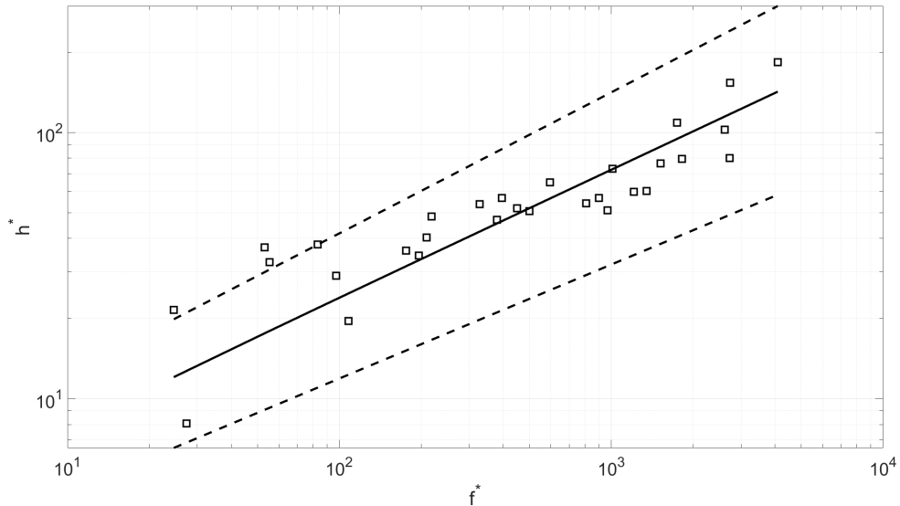
Figure 40. Non-dimensional crater depth, h^* , versus non-dimensional fluence, f^* . \lambda = 1064 nm, \tau_p = 28 \mu s, \omega_0 \approx 6.7 \mu m, F : varied, Material: varied, P = 1 atm, T = 300 K.
