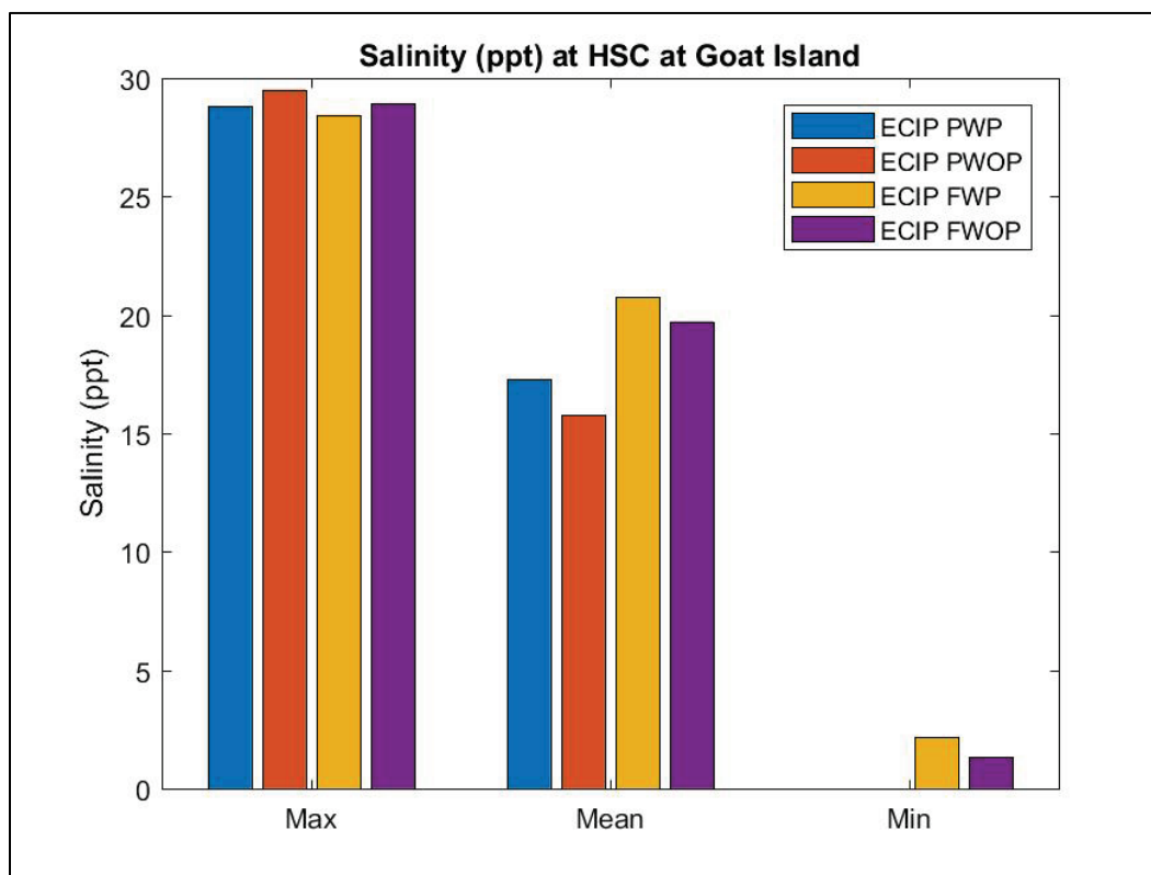
Figure 17. Maximum, minimum, and mean salinity at HSC at Goat Island.
