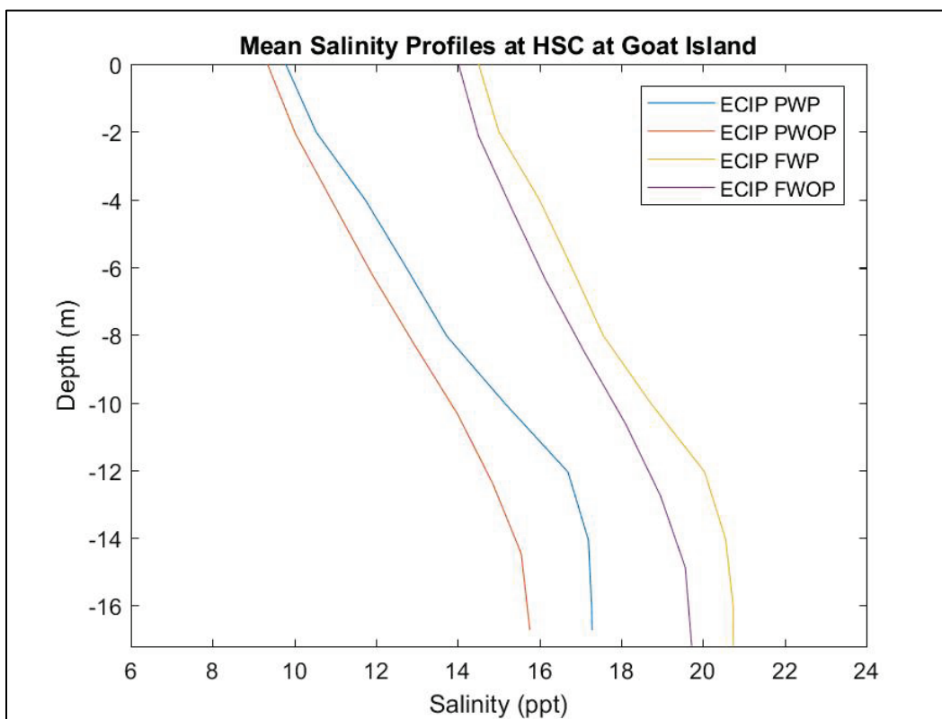
Figure 19. Vertical salinity profile at HSC at Goat Island.
