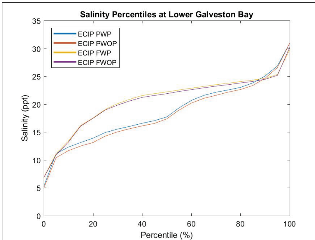
Figure 26. Percent-less-than salinity at HSC at Lower Galveston Bay.
