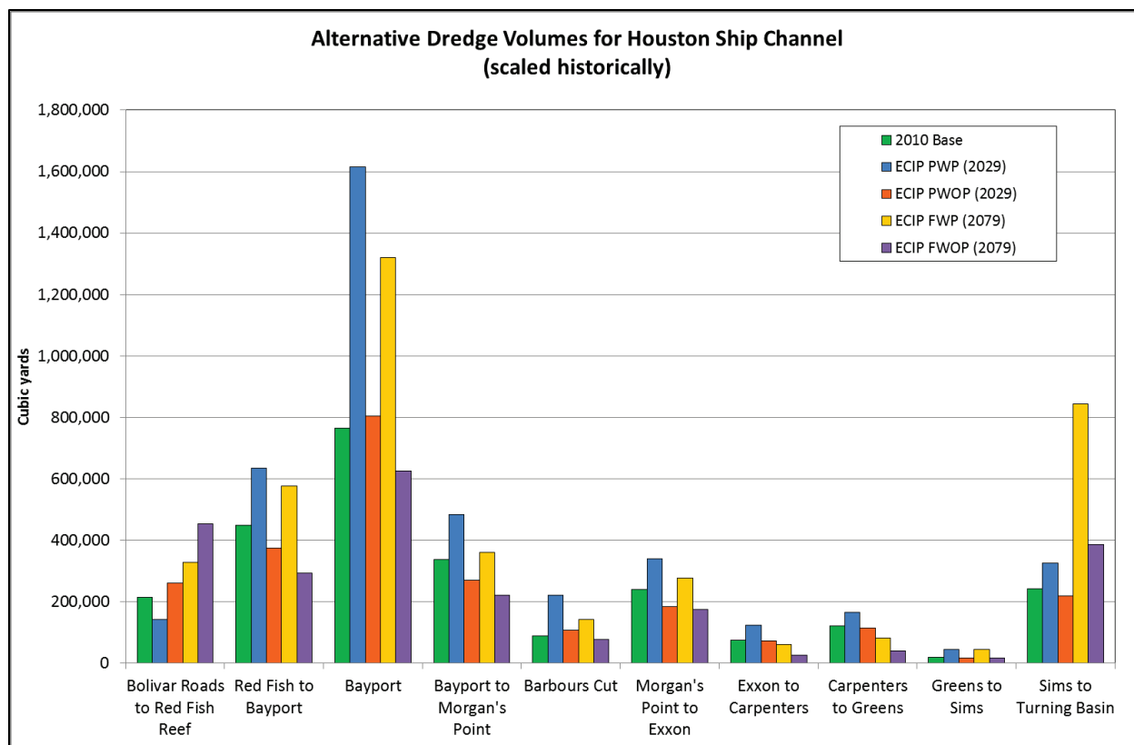
Figure 57. Shoaling results by reach for all alternatives.
