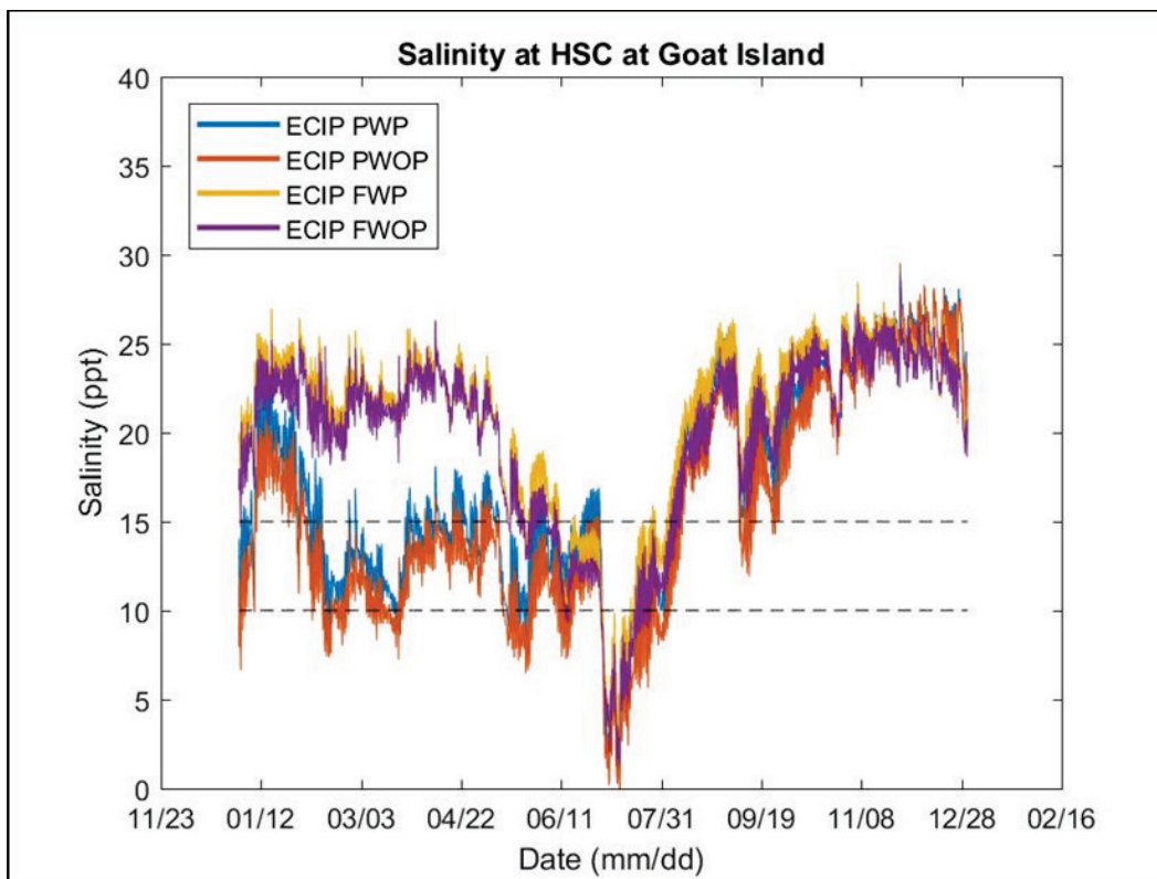
Figure 16. Salinity time history at HSC at Goat Island.
