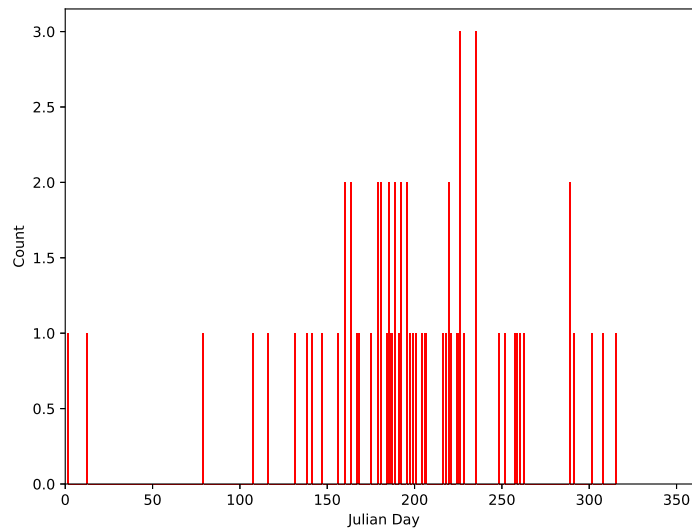
Figure 12. Histogram of the cases organized by Julian day.
