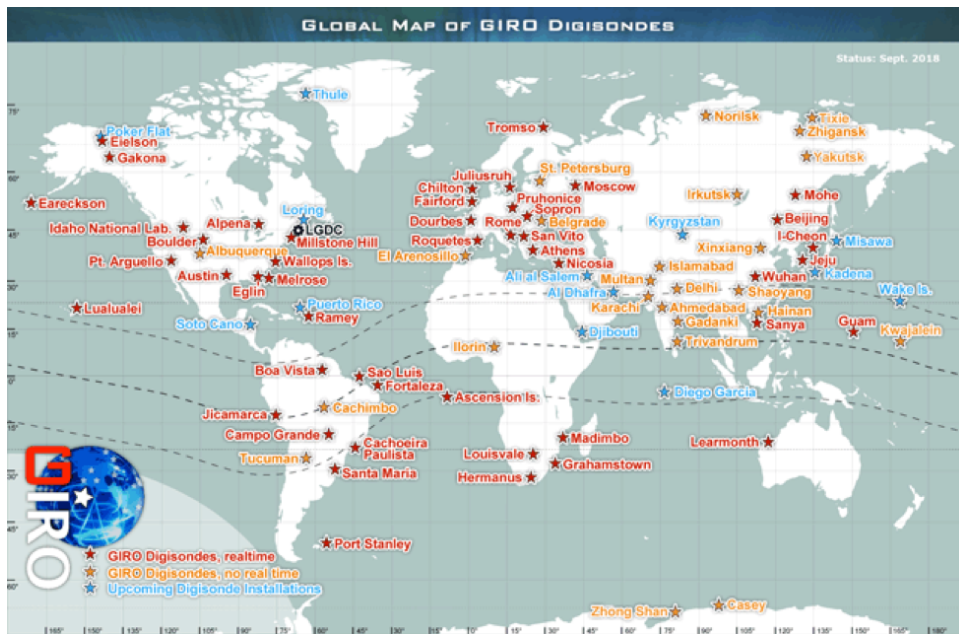
Figure 6. The global coverage of the GIRO Digisonde network as of September 2018 (Center, 2018).
