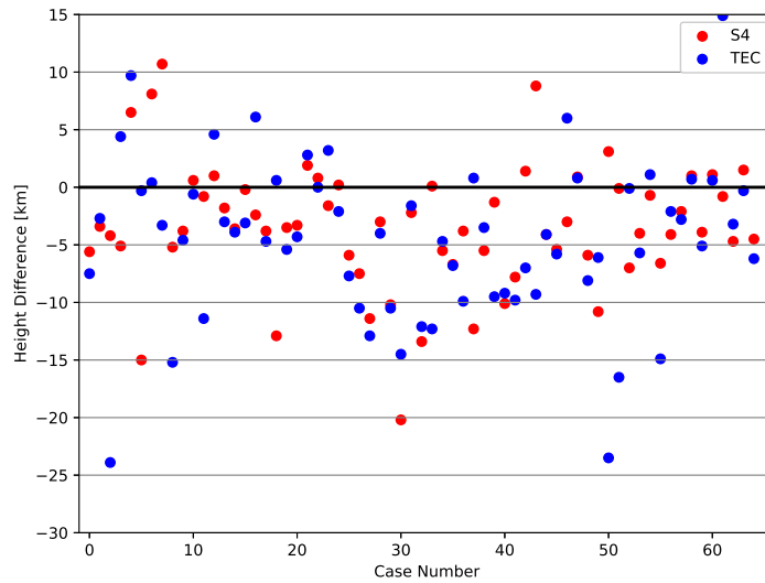
Figure 45. The difference between the calculated Digisonde height and estimated height for each case.
