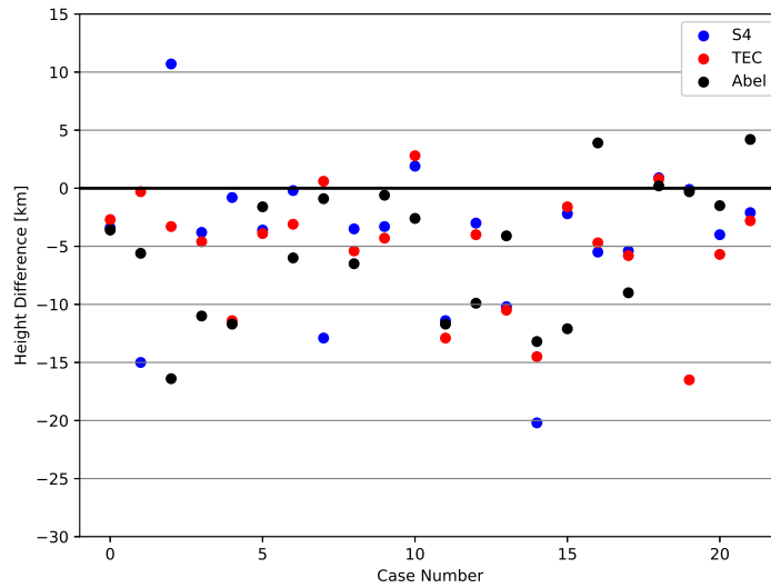
Figure 51. The difference between the calculated Digisonde height and estimated height for each case.
