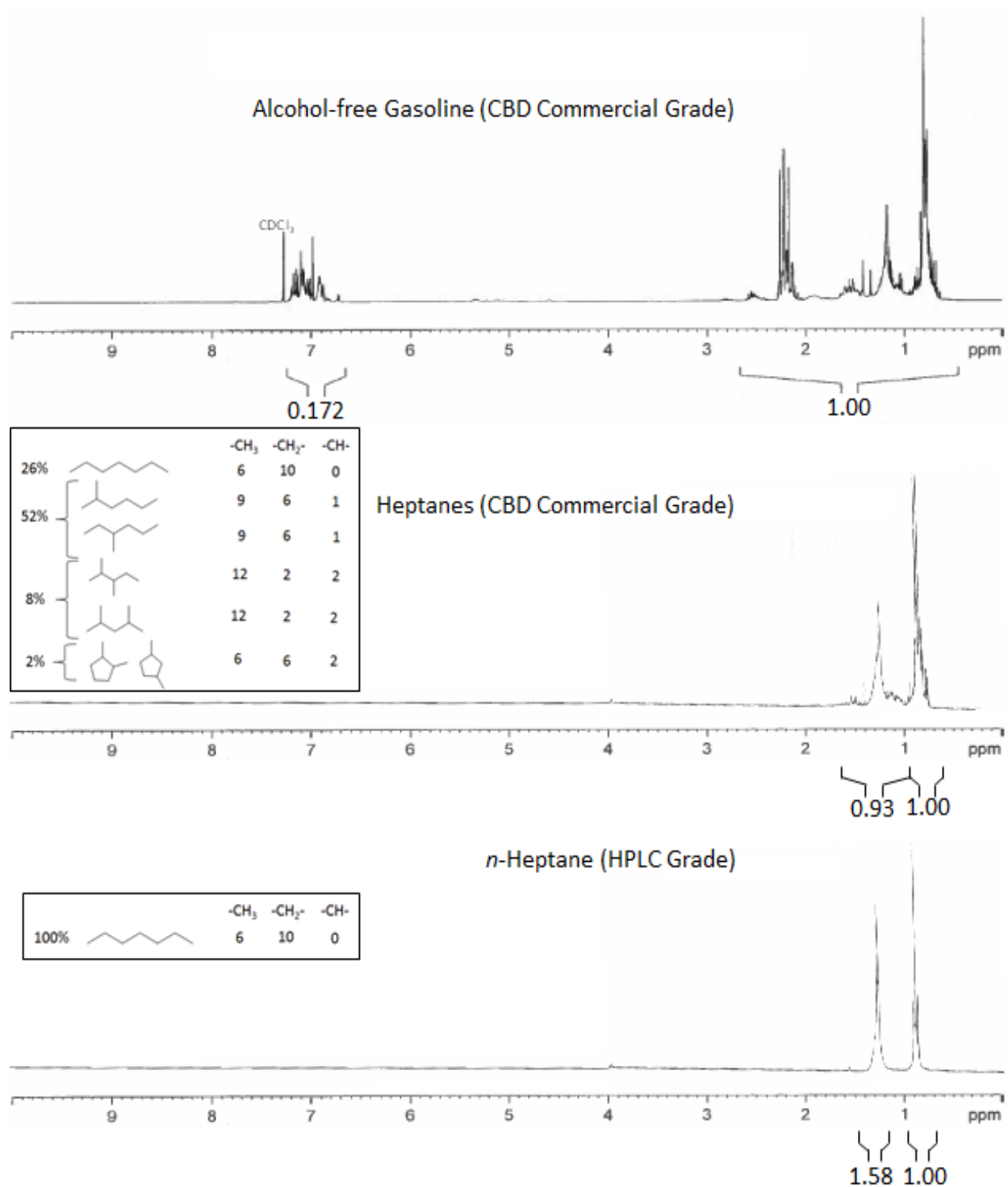
Figure 6. 1 H NMR spectra of alcohol-free gasoline, heptanes and n -heptane used in 28 ft 2 and benchtop pool-fire extinction testing. Integrations are discussed in the text. The inserts on the heptanes and n -heptane spectra identify quantities of major components [41] and the number of methyl, methylene and methane structural units in each component.
