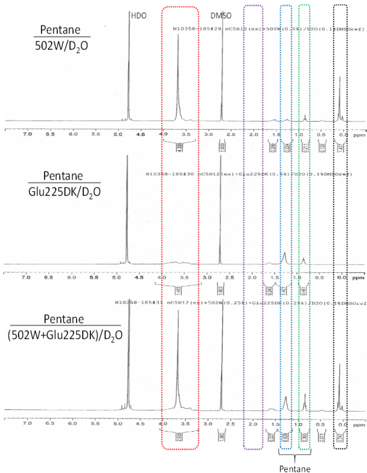
Figure C4. Integrated 1 H NMR spectra of the D 2 O phase of 502W, Glucopon 225DK and the 1:1 combination solutions after 5.0 minutes contact with pentane and low speed stirring.
