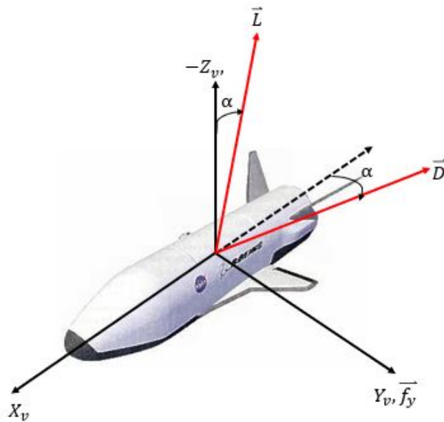
Figure 2. Angle-of-Attack Description
