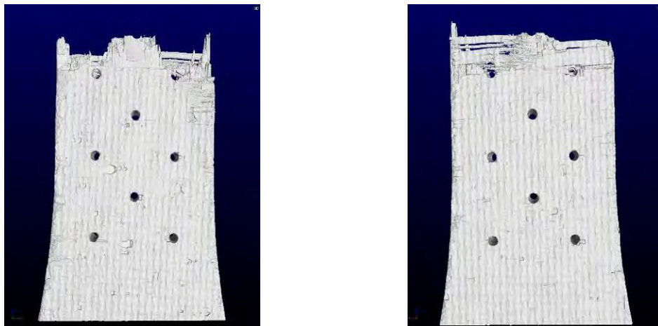
Figure B. 43: 3D image of the top fracture surface of specimen #10, tested in creep at 1200°C in steam ( \sigma_{cr} = 93 MPa, t_f = 6.05 h)
