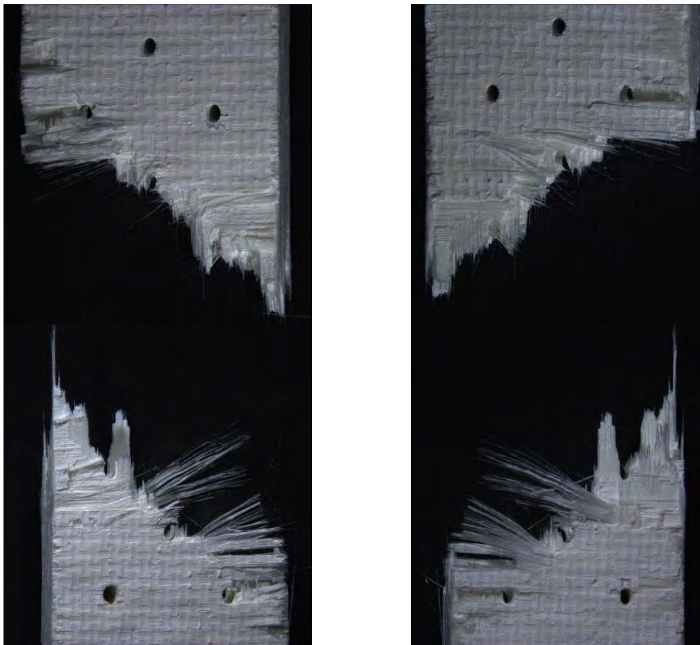
Figure A. 15: Top and bottom fracture surfaces of specimen #7, tested in tension to failure following 100 h creep at 46 MPa at 1200°C in air
