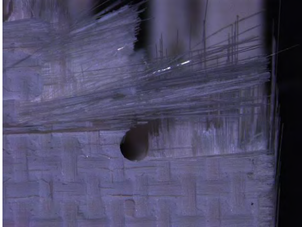
Figure A. 51: Fracture surface of specimen #9, tested in creep at 1200°C in steam ( \sigma_{cr} = 116 MPa, t_f = 0.61 h)
