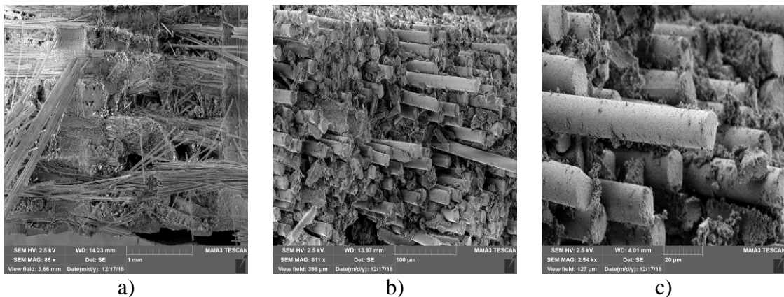
Figure D. 16: Fracture surface of specimen #12 (Area 2), tested in tension to failure following 100 h creep at 46 MPa at 1200°C in steam: (a) 88X, (b) 811X, (c) 2.5kX
