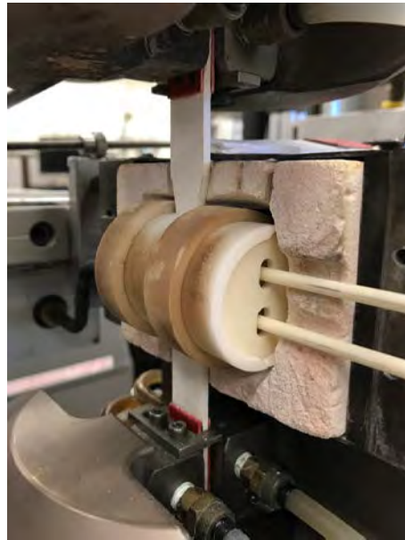
Figure 12: Alumina susceptor
