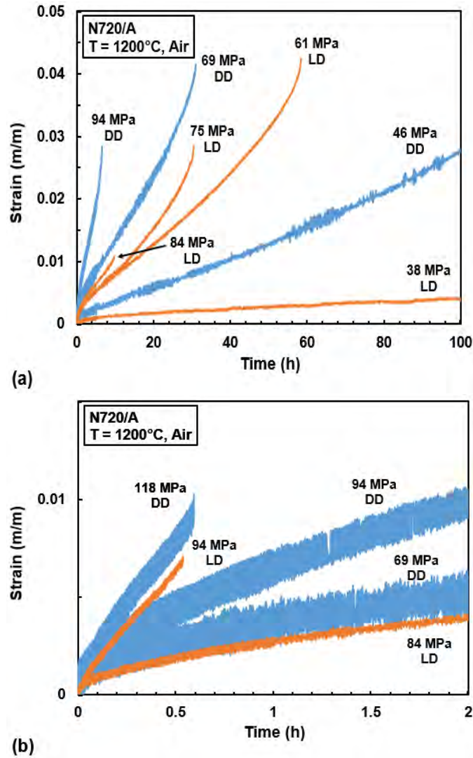
Figure 25: Creep strain vs time curves obtained for N720/A specimens with diamond-drilled and laser-drilled holes in air at 1200°C: (a) time scale selected to show creep curves obtained at 38-94 MPa, and (b) time scale selected to show creep curves obtained at higher creep stresses
