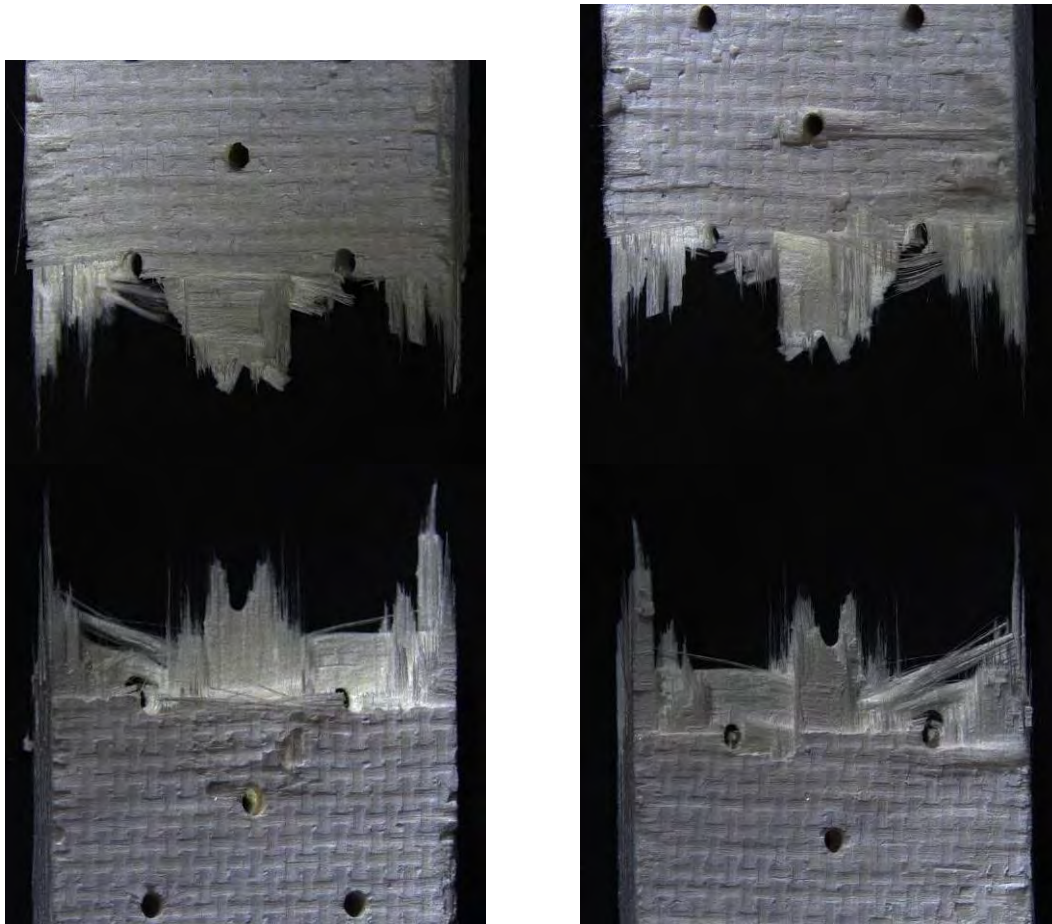
Figure A. 25: Top and bottom fracture surfaces of specimen #5, tested in creep at 1200°C in air ( \sigma_{cr} = 94 MPa, t_f = 6.55 h)
