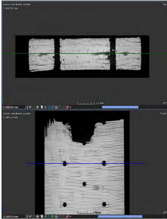
Figure B. 28: 2D (x-z plane) vs 2D (x-y plane) location showing damage zone at Step 4 for specimen #6, tested in creep at 1200°C in air ( \sigma_{cr} = 69 MPa, t_f = 30.95 h)
