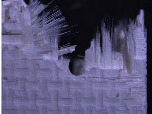
Figure A. 43: Fracture surface of specimen #12, tested in tension to failure following 100 h creep at 46 MPa at 1200°C in steam
