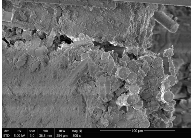
Figure C. 3: Fracture surface of specimen #3, tested in tension to failure at 1200°C in air
