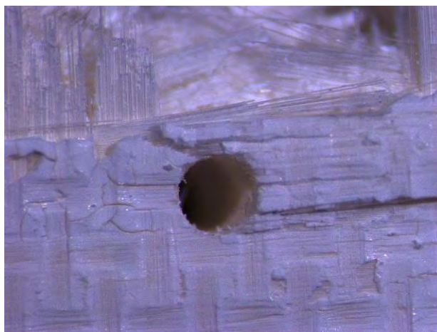
Figure A. 61: Fracture surface of specimen #11, tested in creep at 1200°C in steam ( \sigma_{cr} = 150 MPa, t_f = 0.04 h)
