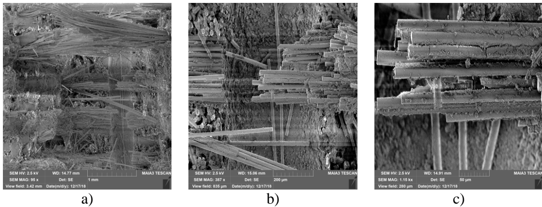
Figure D. 15: Fracture surface of specimen #12 (Area 1), tested in tension to failure following 100 h creep at 46 MPa at 1200°C in steam: (a) 95X, (b) 387X, (c) 1kX
