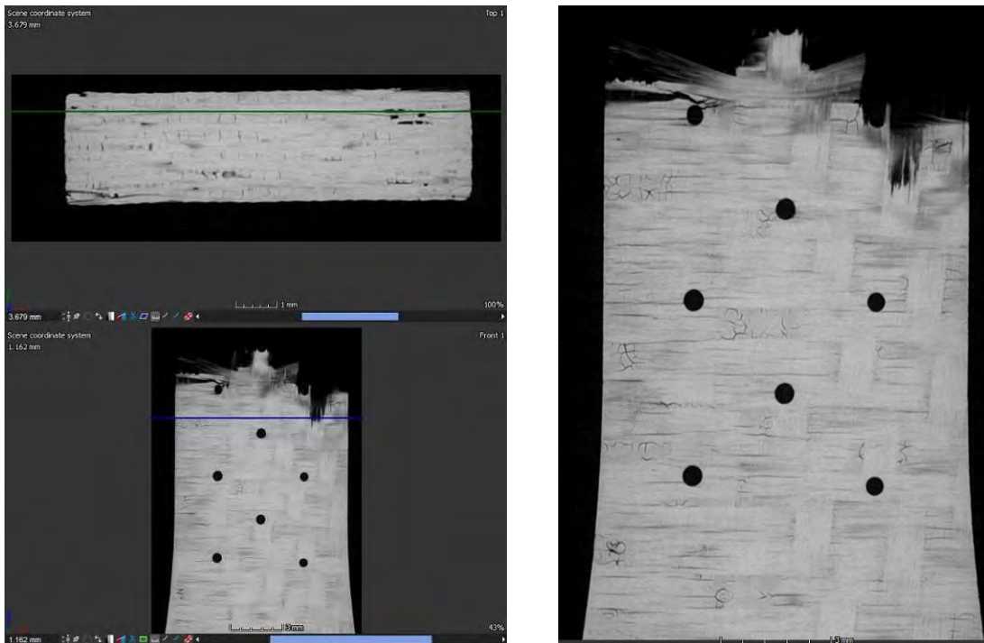
Figure B. 41: 2D (x-z plane) vs 2D (x-y plane) location showing damage zone at Step 3 for specimen #12, tested in tension to failure following 100 h creep at 46 MPa at 1200°C in steam
