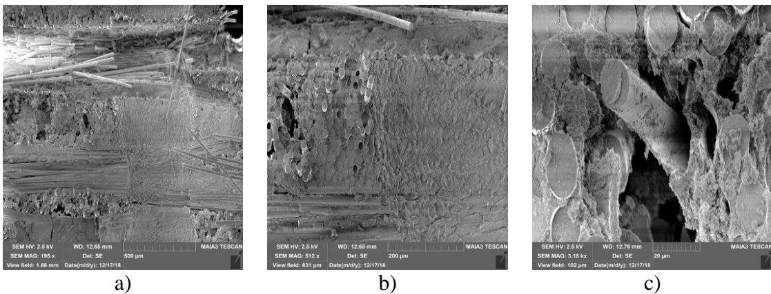
Figure D. 29: Fracture surface of specimen #11 (Area 2), tested in creep at 1200°C in steam ( \sigma_{cr} = 150 MPa, t_f = 0.04 h): (a) 195X, (b) 512X, (c) 3kX
