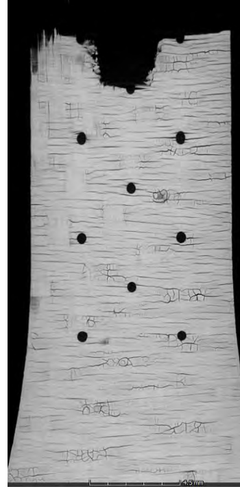
Figure B. 28: 2D (x-z plane) vs 2D (x-y plane) location showing damage zone at Step 4 for specimen #6, tested in creep at 1200°C in air ( \sigma_{cr} = 69 MPa, t_f = 30.95 h)
