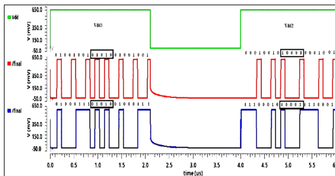
Fig. 3. Simulation Result of the Authentication Circuit
