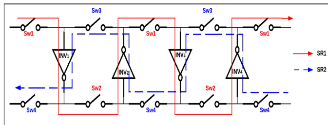
Fig. 2. Merged PUF/Dynamic Shift Register
