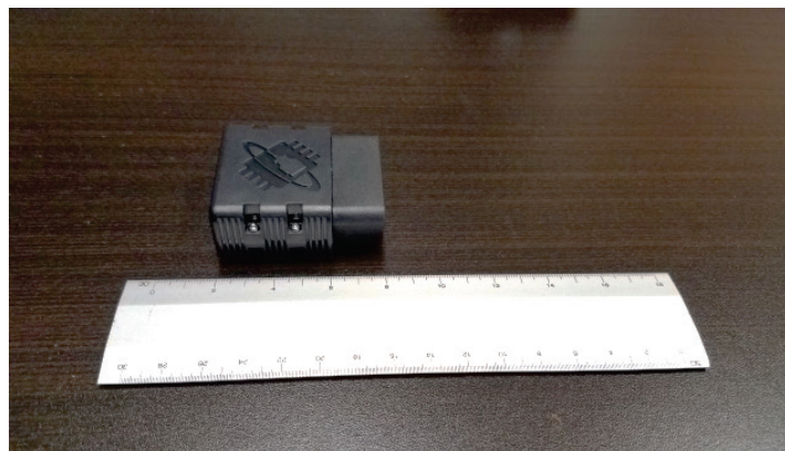
b) OBDLink MX Bluetooth Scan Tool (2.0 x 1.7 x 0.8 in.)
