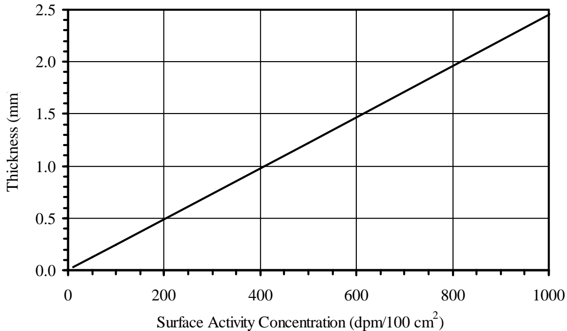
Figure D-1. Averaging Thickness of Concrete vs. Mean Surface Concentrations of 239+240 Pu at 8 pCi/g.
