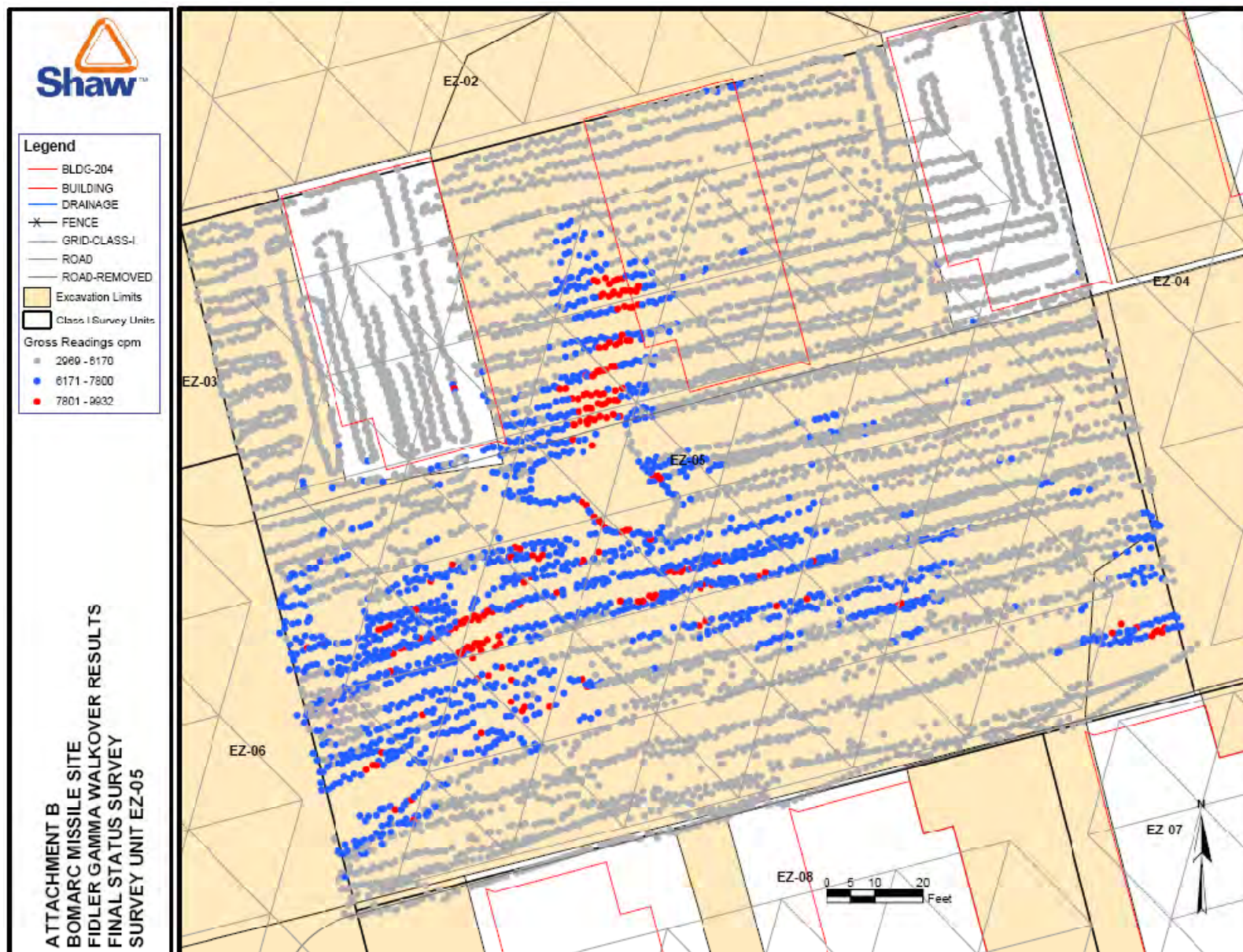
Figure B-6. Example FIDLER Scan Data for Survey Unit EZ-5 (Duratek 2005).
