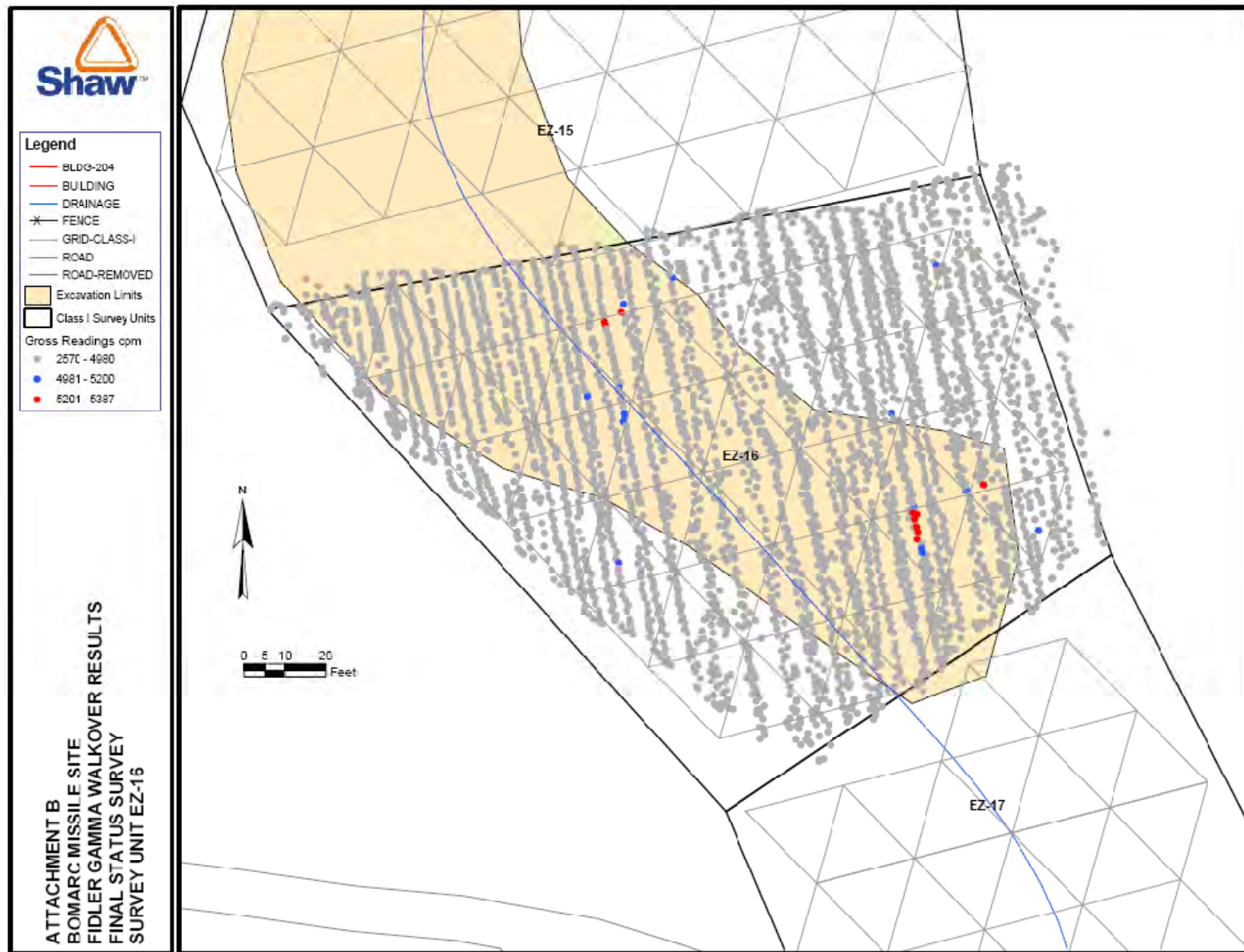
Figure B-7. Example FIDLER Scan Data for Survey Unit EZ-16 (Duratek 2005).
