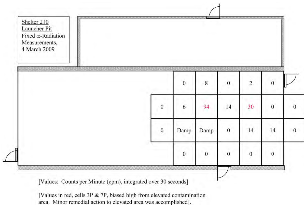
Figure E-3. Fixed \alpha -Radiation Measurements in Launcher Pit of Shelter 210 [Appendix F, Rademacher et al. (2009)].
