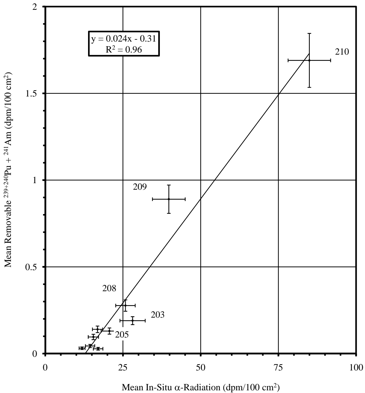
Figure D-7. Scatter plot of Mean Removable 239+240 Pu + 241 Am Concentration to Mean In-Situ \alpha -Radiation Concentration [Annotation of Select Shelters, 1- \sigma Uncertainty Bars] (Rademacher et al. 2009).
