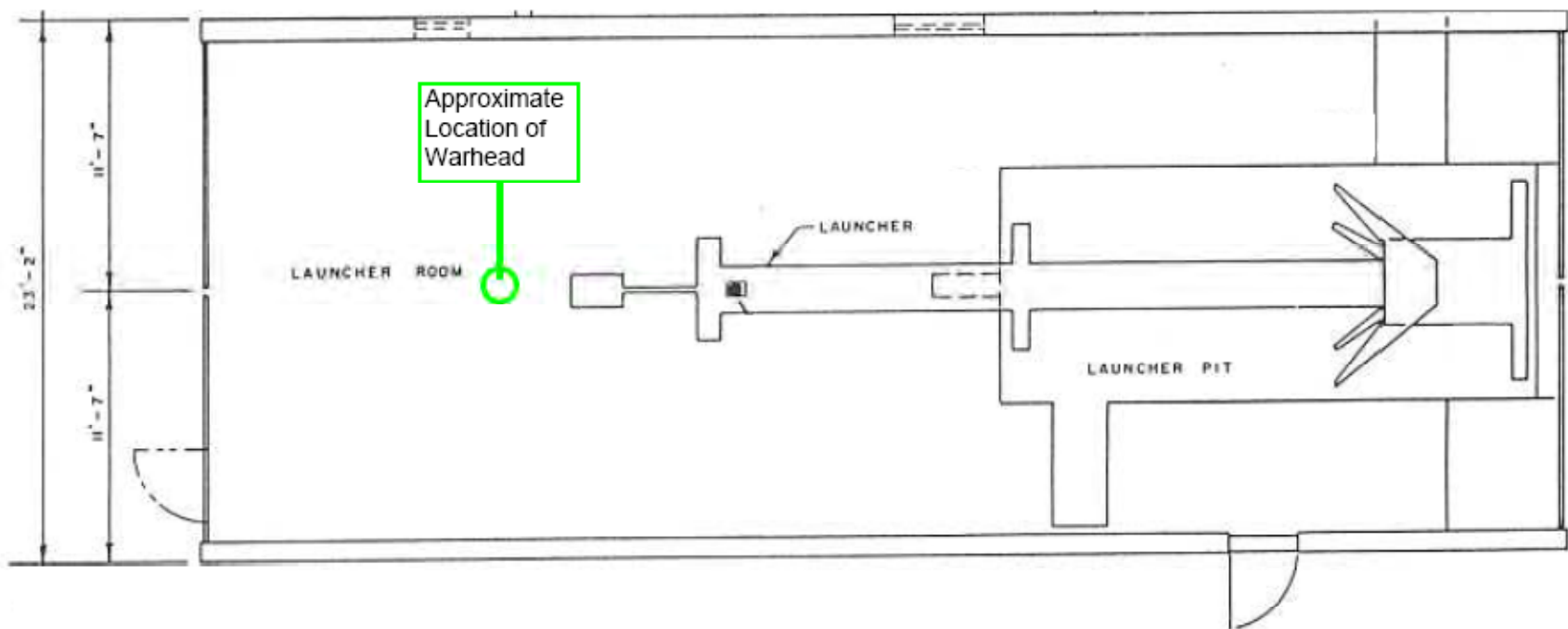
Figure A-3. Dimensions of Shelter Showing Simple Detail of Launcher Pit, Launcher, and Warhead Locations.
