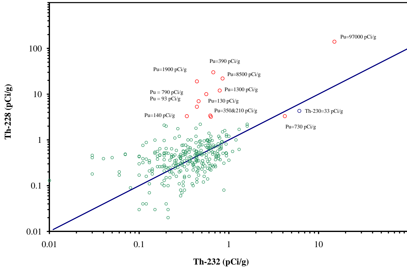
Figure A-9. ^{228}\text{Th} vs. ^{232}\text{Th} Concentrations for Samples Analyzed during the 1997 OHM Characterization Study [Atch 2, Rademacher (1999c)].
