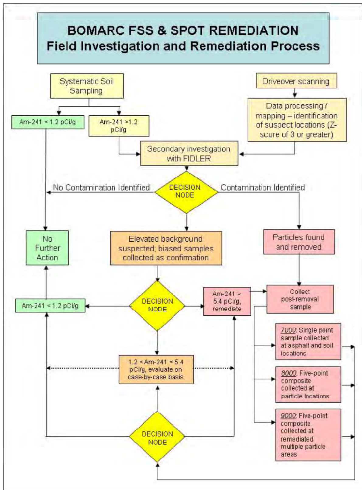
Figure C-13. Investigation, Remediation, and Resurvey Process Used for Secondary Areas (Cabrera 2008).
