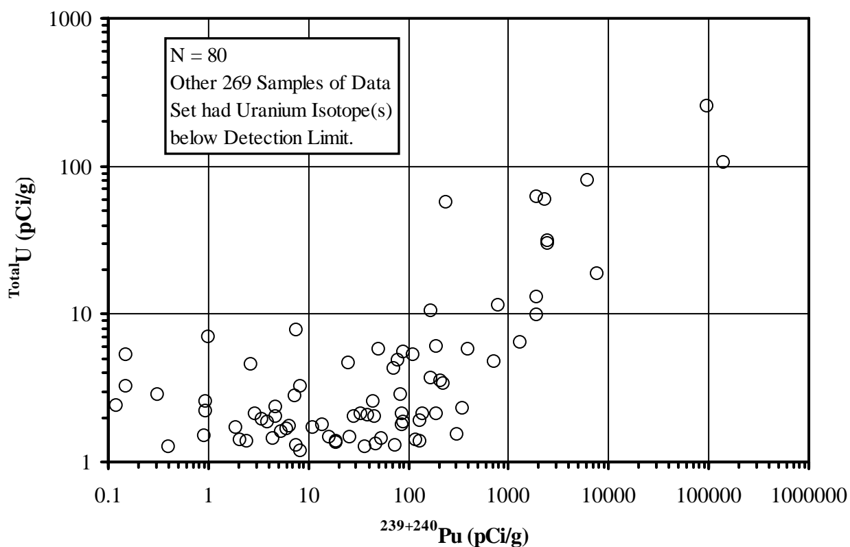
Figure A-7. Alpha Spectroscopy Data from 1997 Characterization (OHM 1998).
