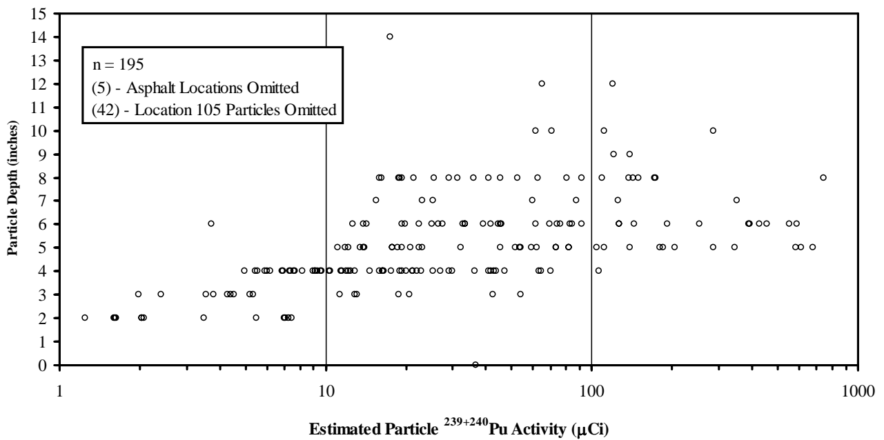
Figure C-8. Estimated Particle 239+240 Pu Activities vs. Depth (Data from Cabrera 2006a).
