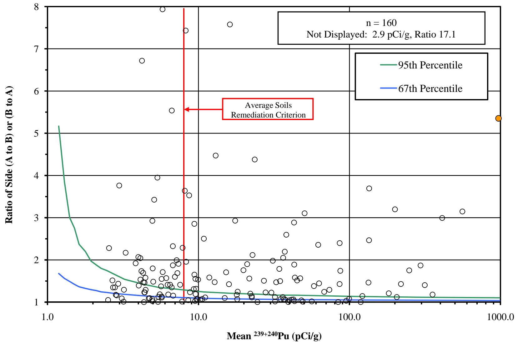
Figure C-21. Ratios of Activity Concentration for Conjugate Assessment of Select Final Status and Biased Soil Samples [Data from Cabrera (2008)].
