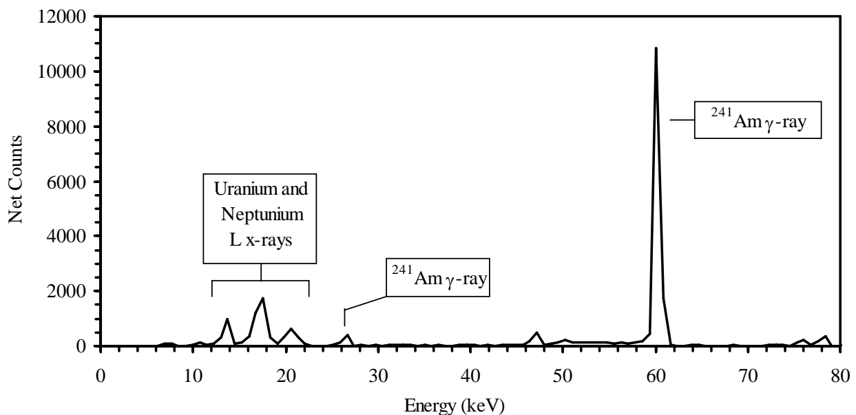
Figure A-5. Low-Energy Germanium Spectra for Discrete Particle Removed from a Shelter (Favret 2007).
