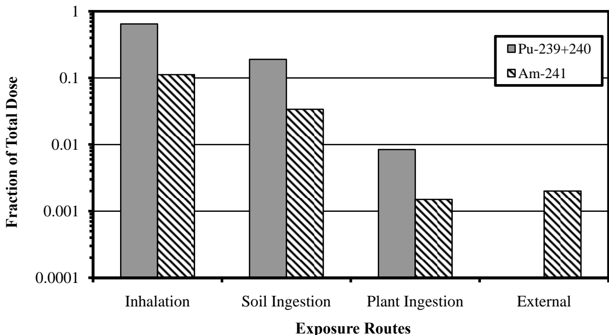
Figure 2-2. RESRAD Exposure Route Summary for t = 0 [Data from RI/FS, Appendix J, Earth Tech (1992)]. [Note: ^{241}\text{Am} Modified for ^{239+240}\text{Pu} to ^{241}\text{Am} Ratio of 5.4].
