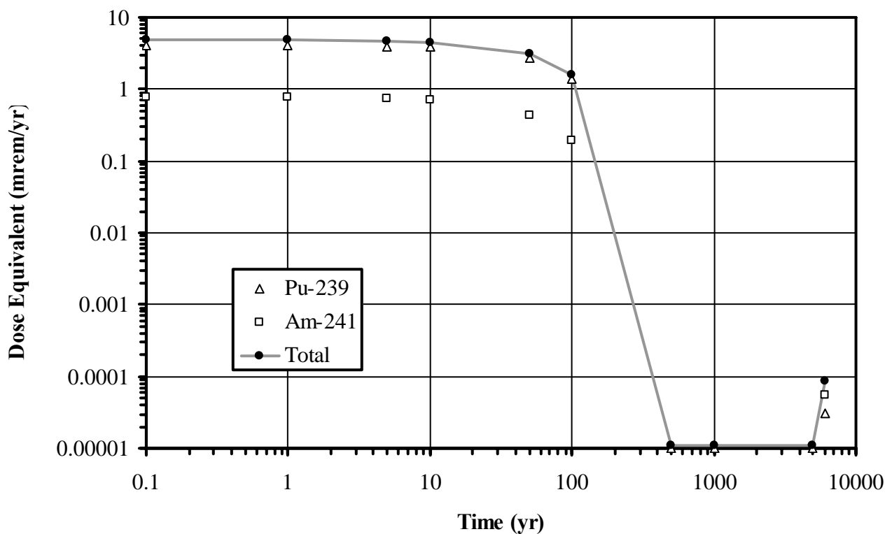
Figure 2-1. RESRAD Dose Summary Over Time [Data from RI/FS, Appendix J, Earth Tech (1992)]. [Note: ^{241}\text{Am} Modified for ^{239+240}\text{Pu} to ^{241}\text{Am} Ratio of 5.4, and Average ^{239+240}\text{Pu} Concentration of 8 pCi/g].
