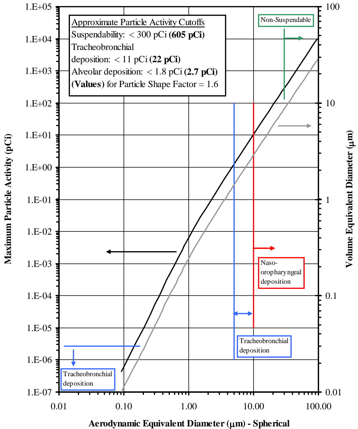
Figure C-11. Maximum Particle Activities and Volume Equivalent Diameters for Aerodynamic Equivalent Diameter (Spherical) \text{PuO}_2 Particles.
