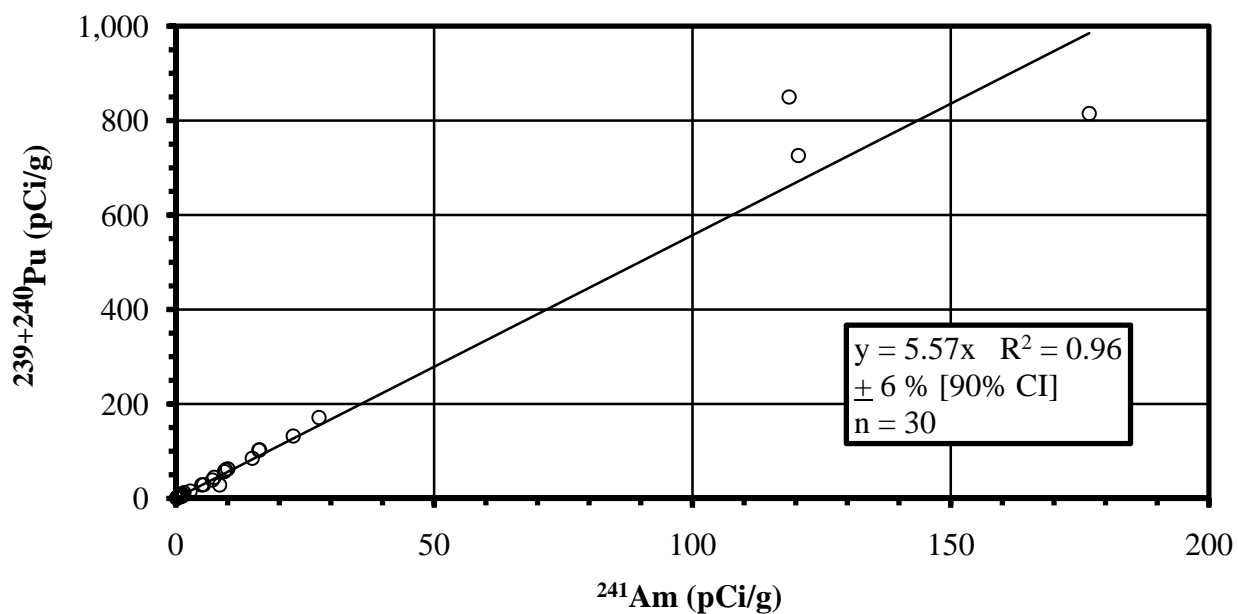
Figure A-8. ^{239+240}\text{Pu} vs. ^{241}\text{Am} \alpha -Spectroscopy [Data from Duratek (2006)].
