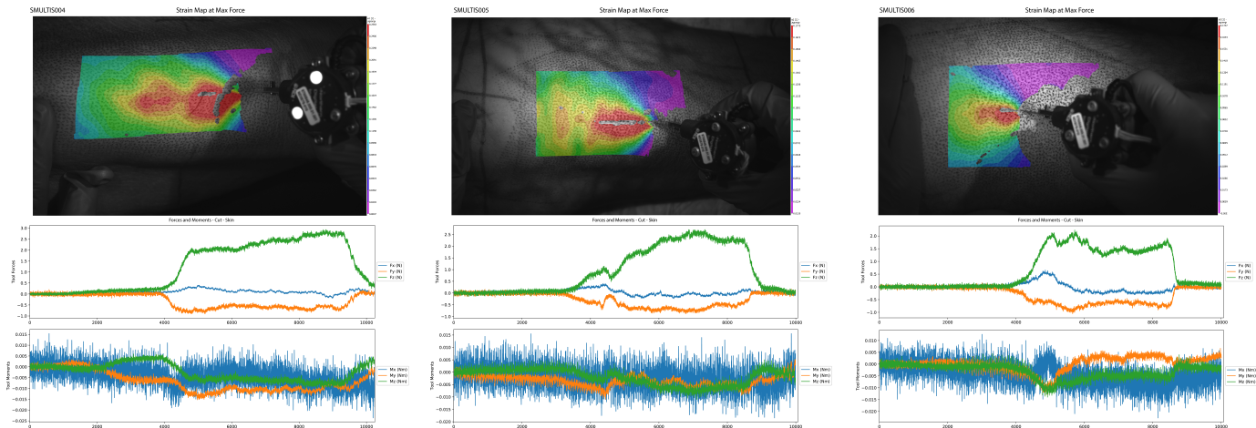
Figure 3. Strain map and cutting forces during the use of a scalpel on three upper leg specimens; strain distributions at peak force are shown.
