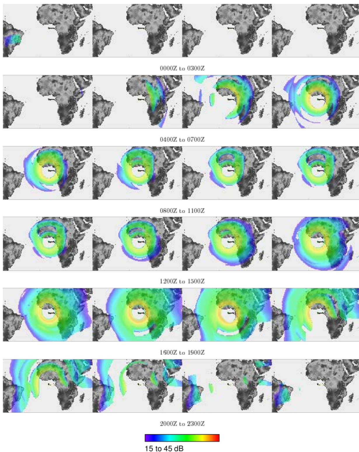
Figure D-3. 24 hour forecast of a 13.0 MHz signal.
