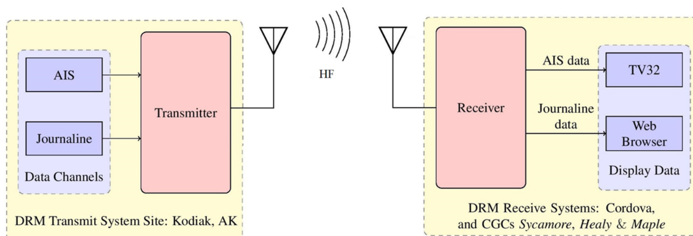
Figure 3. Block diagram of the DRM transmit and receive systems.
