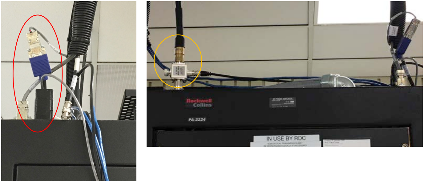
Figure B-5. Transmitter antenna interlock circled in red (left) and installed RF tap circled in orange (right).
