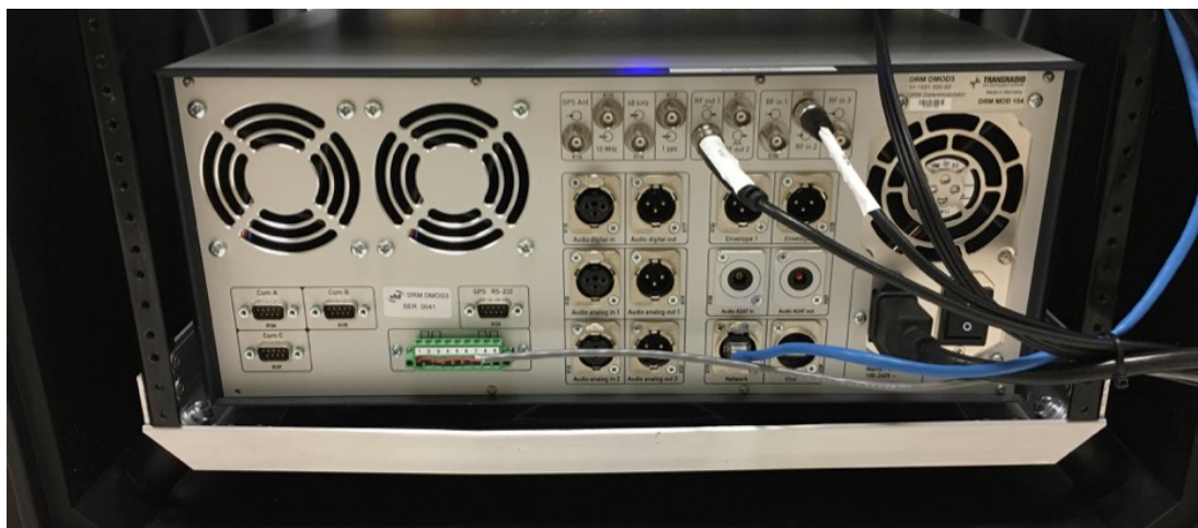
Figure B-6. Back of DMOD3 showing RF output and RF input connections.
