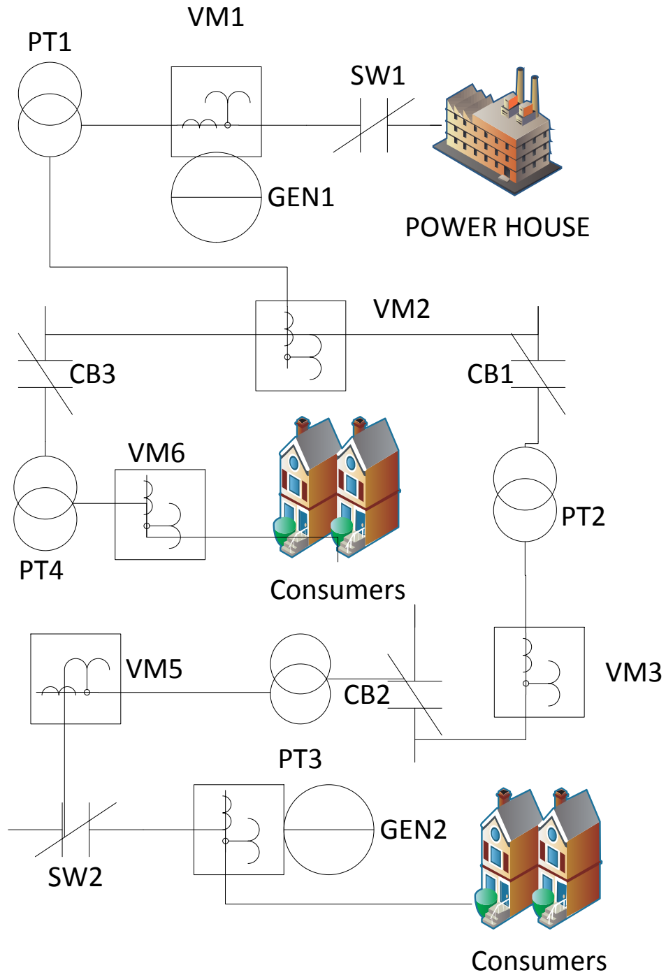
Figure 6: Schematic diagram of the power transmission and distribution simulator
